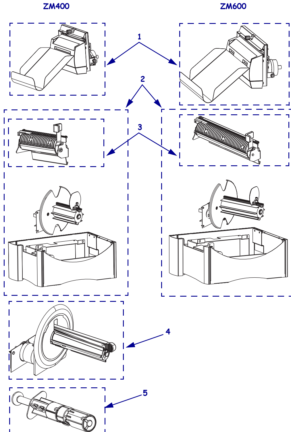
Figure S • Available Media Handling Options
