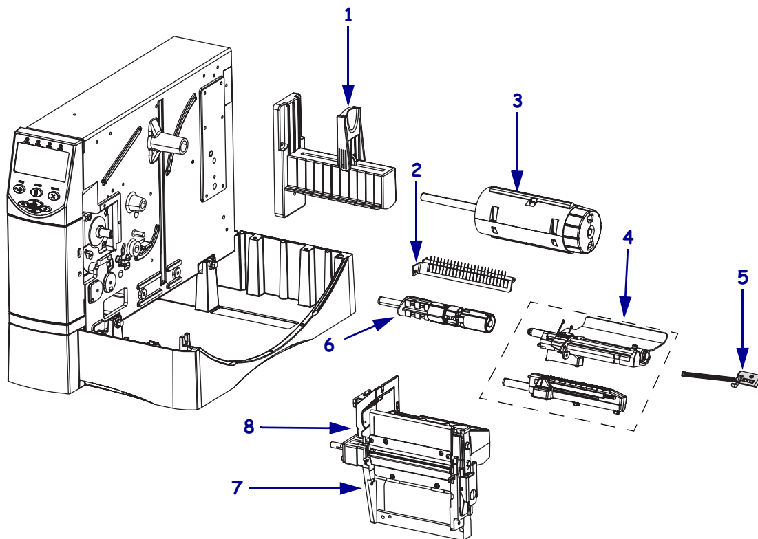
Figure D • Media and Ribbon Path
