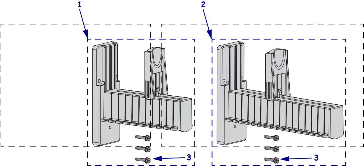
Figure E • Media Hanger
