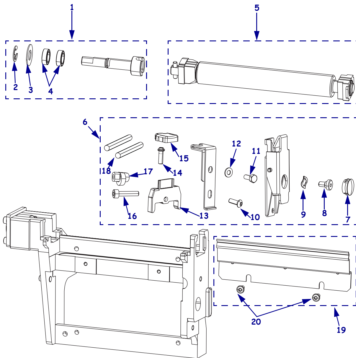
Figure K • Platen Housing
