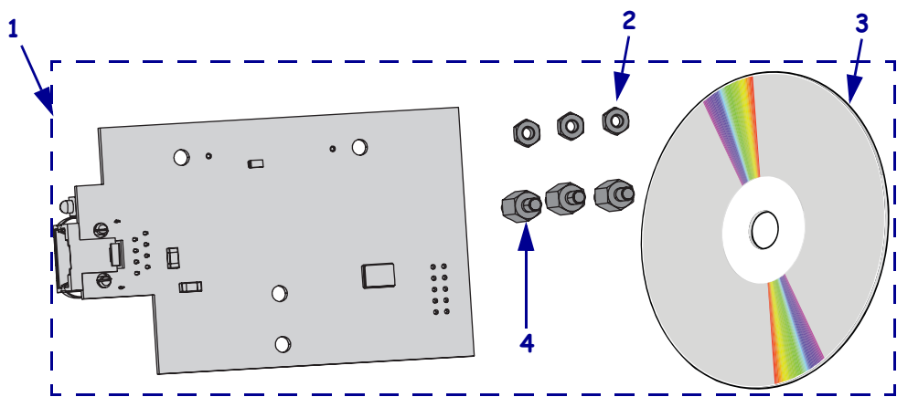
Figure R • Wired Ethernet Board/Internal PrintServer
