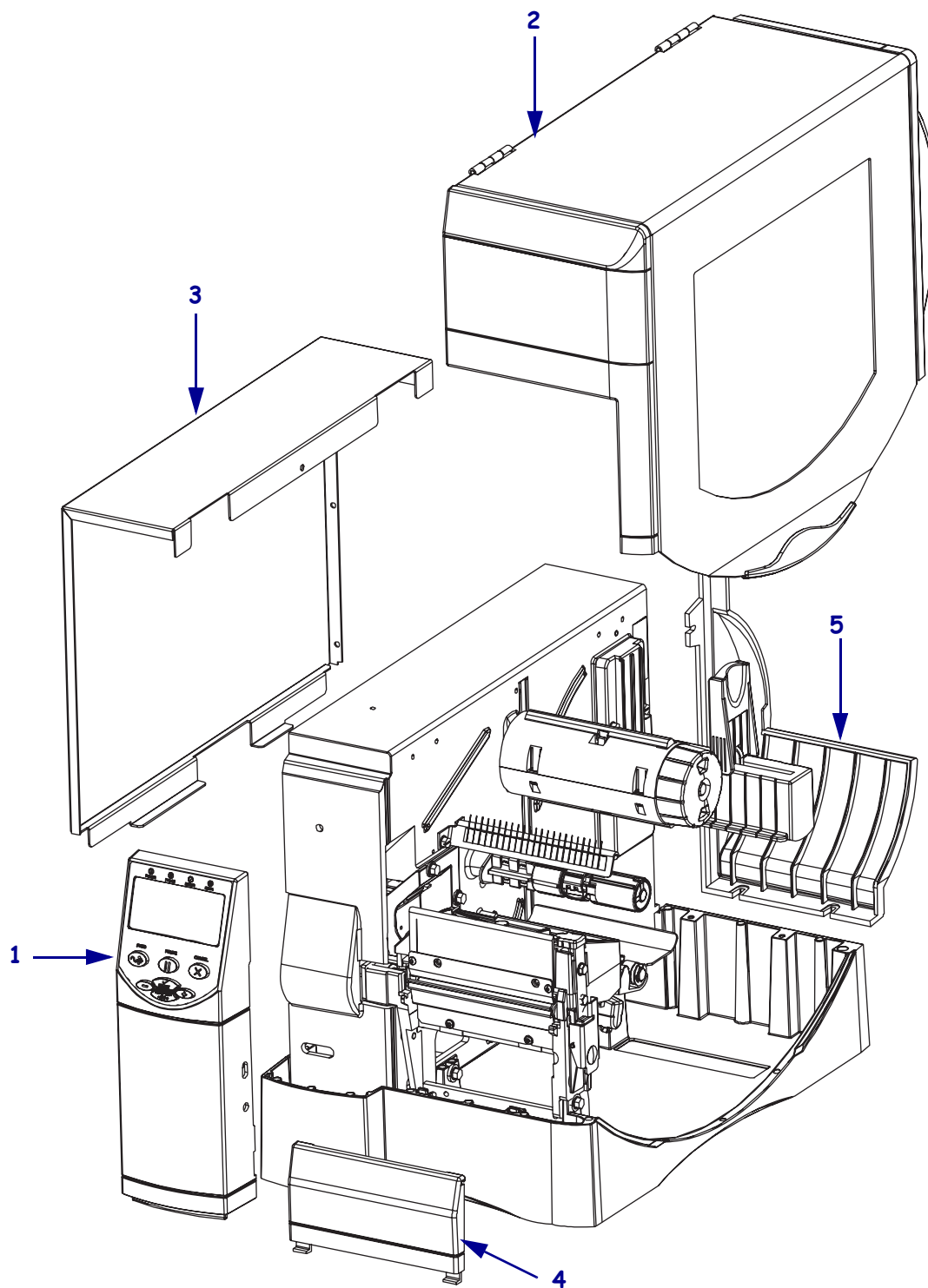
Figure A • Outer Casings
