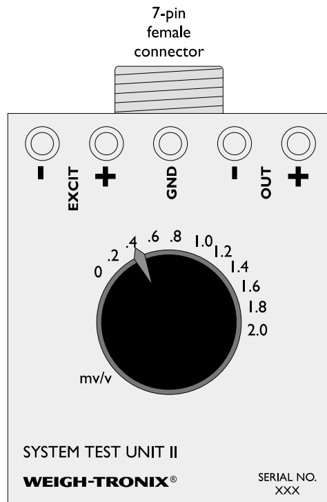
Figure 1 Box A Weight Sensor Simulator
