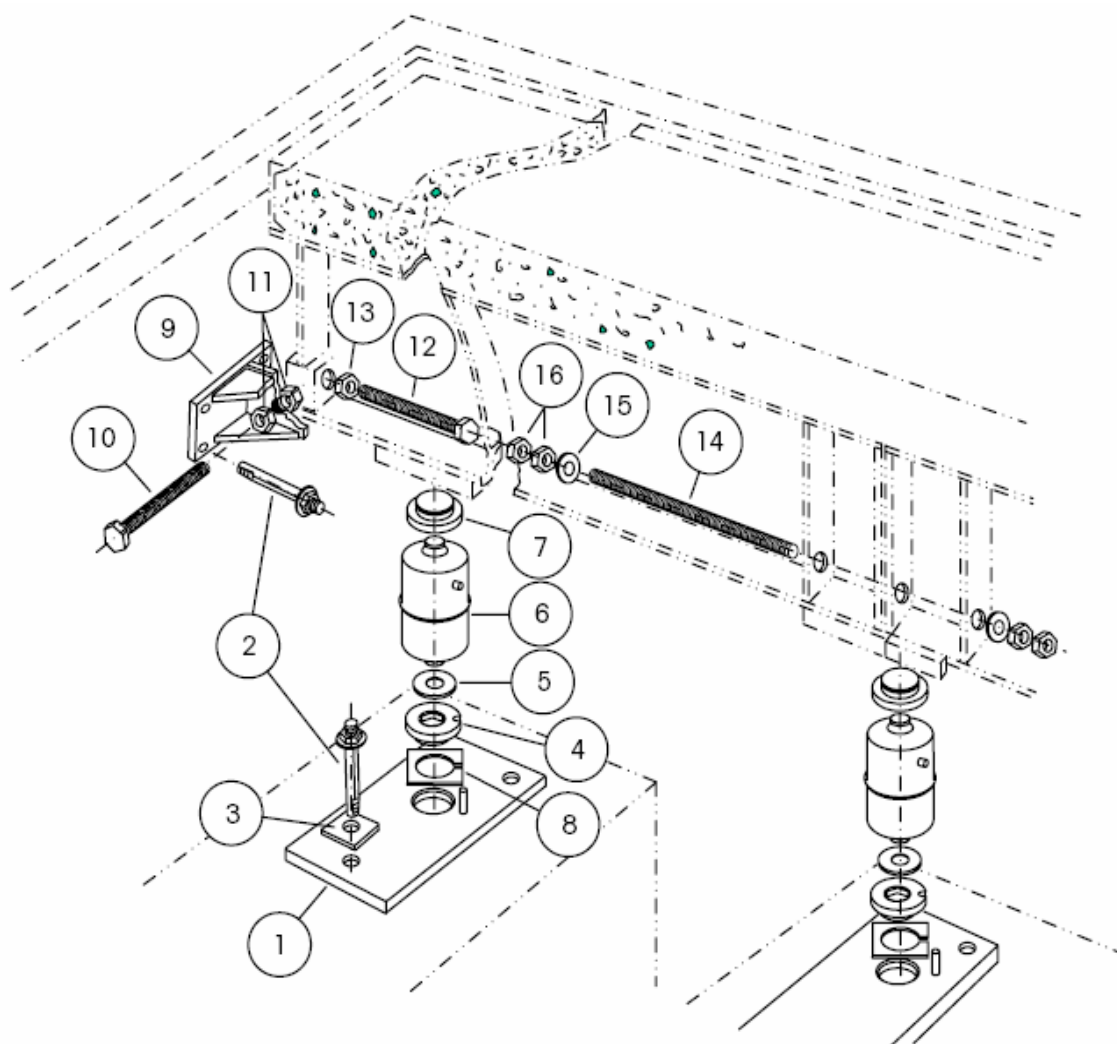
7541 Load Cell Assembly, Tie Rod, and Bumper
