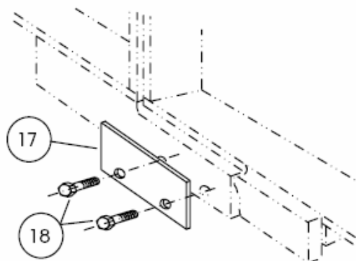
7541 Coupler Side Shim
