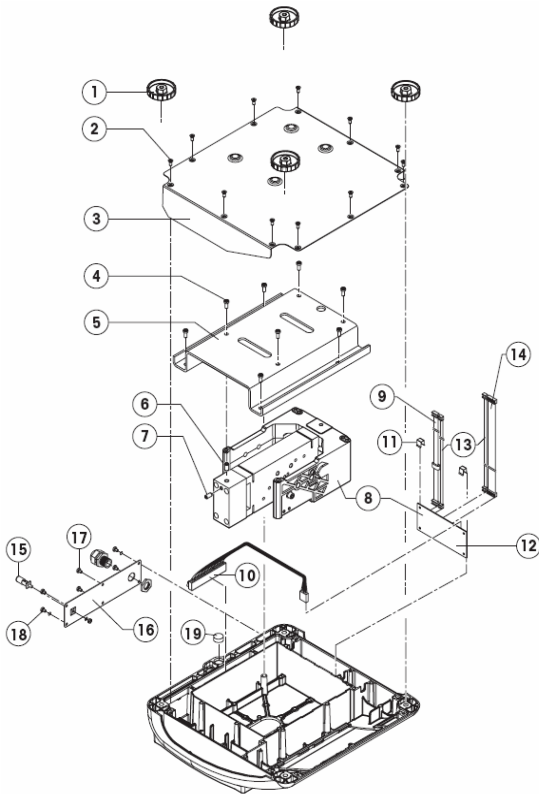
Viper EX - Large Platform MonoBloc Internal View
