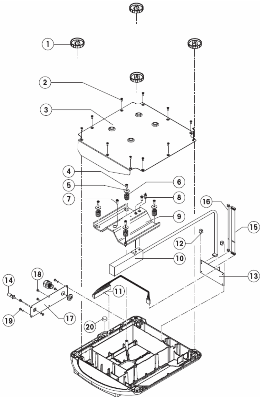
Viper EX - Large Platform Internal View
