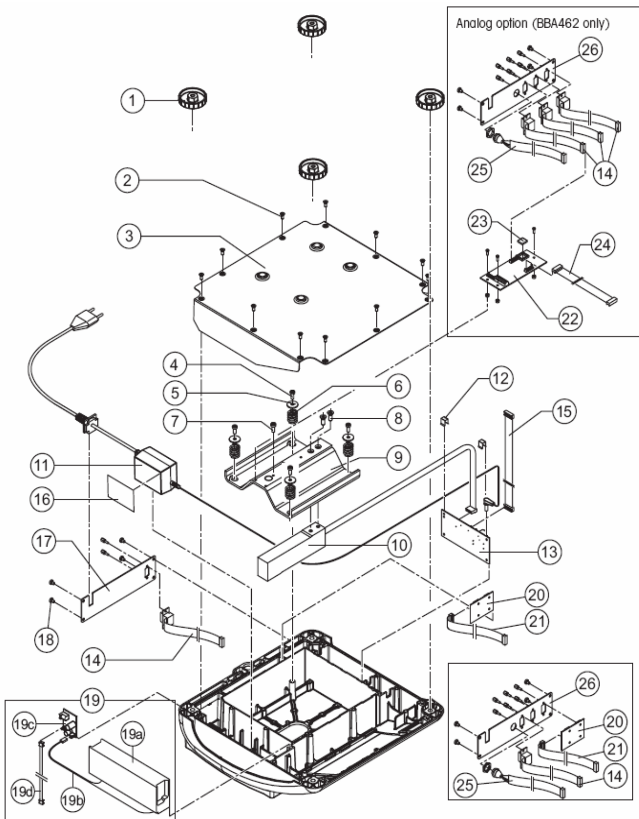
BBA4x2 Large Platform - Interior
