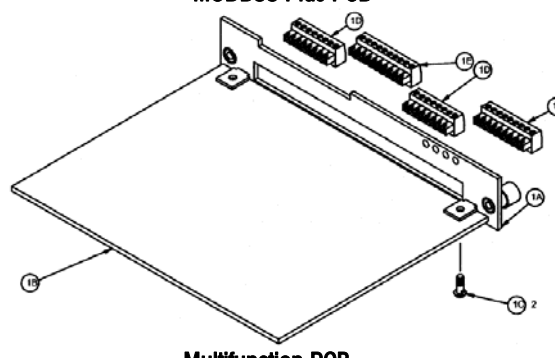
Multifunction PCB
