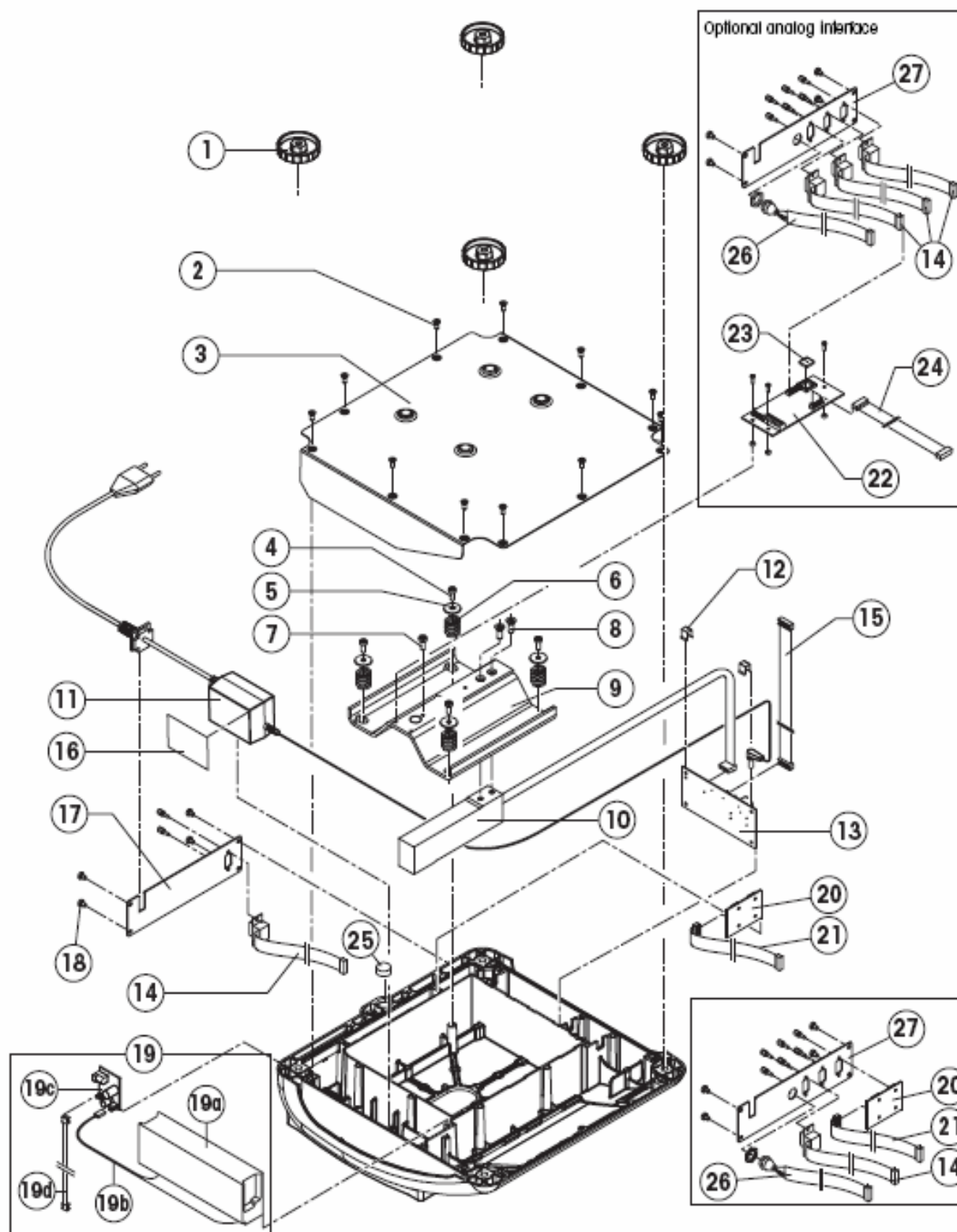
Viper Large Platform - Interior
