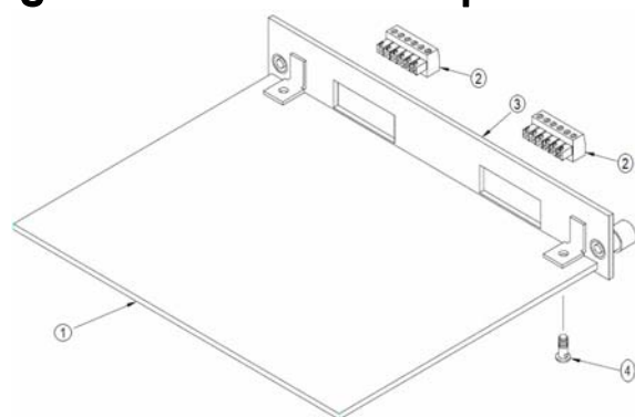
Dual Analog Output Assembly
