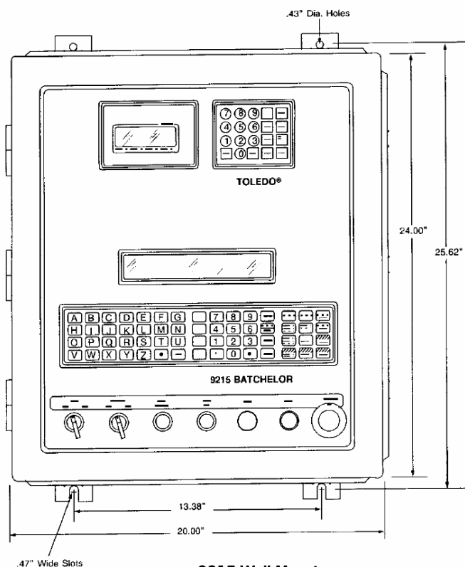
9215 Wall Mount
