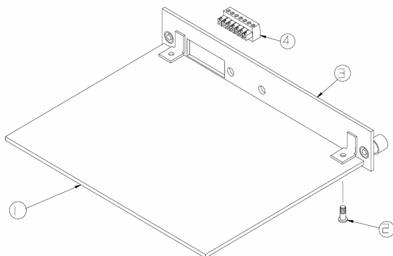
High Precision IDNet PCB Assembly
