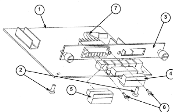
Analog Load Cell PCB
