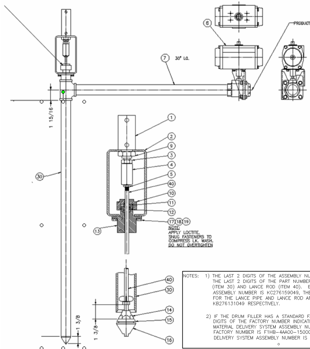
9127 - Material Delivery System (MDS)
