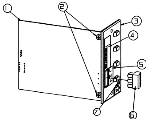
Power Supply
