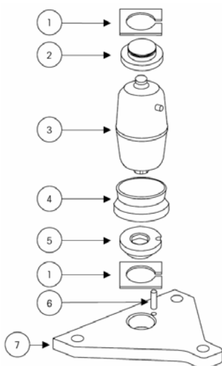
Load Cell Assembly
