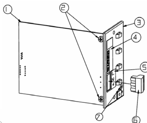
Power Supply Assembly
