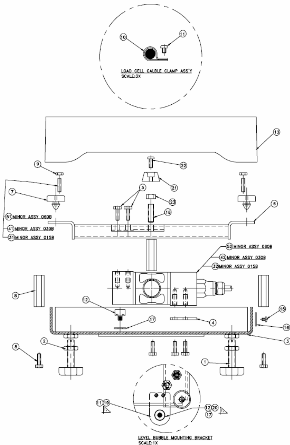
Trimweigh III - 12" Base
