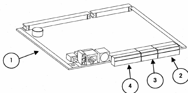
Controller PCB
