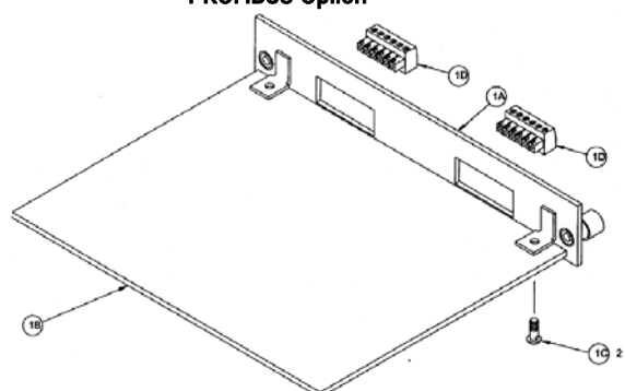
Dual Analog Output Option
