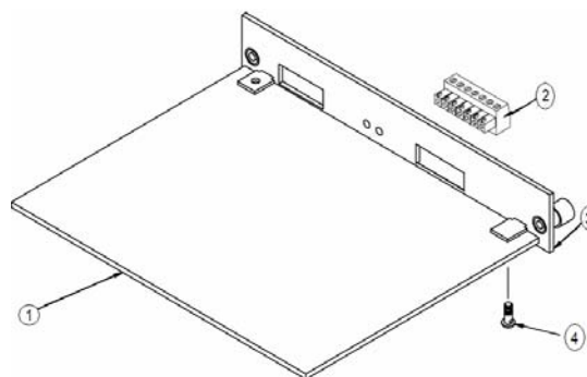
Powercell PCB
