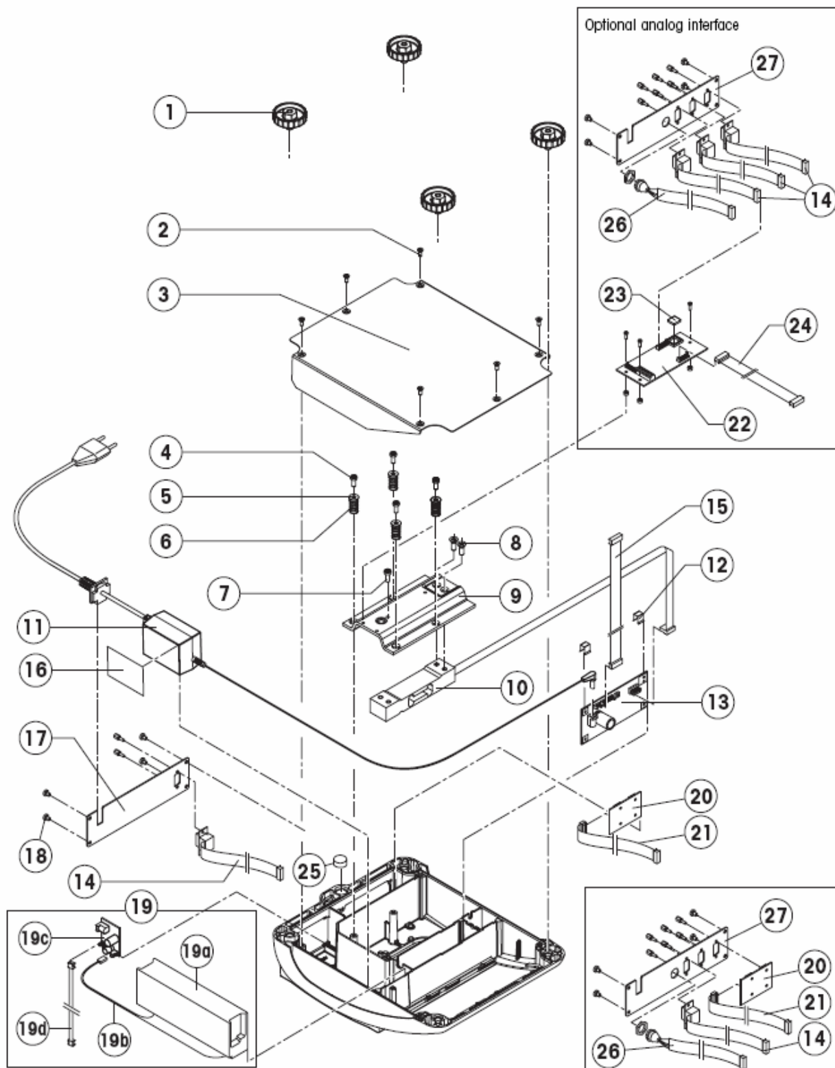
Viper - Small Platform Interior
