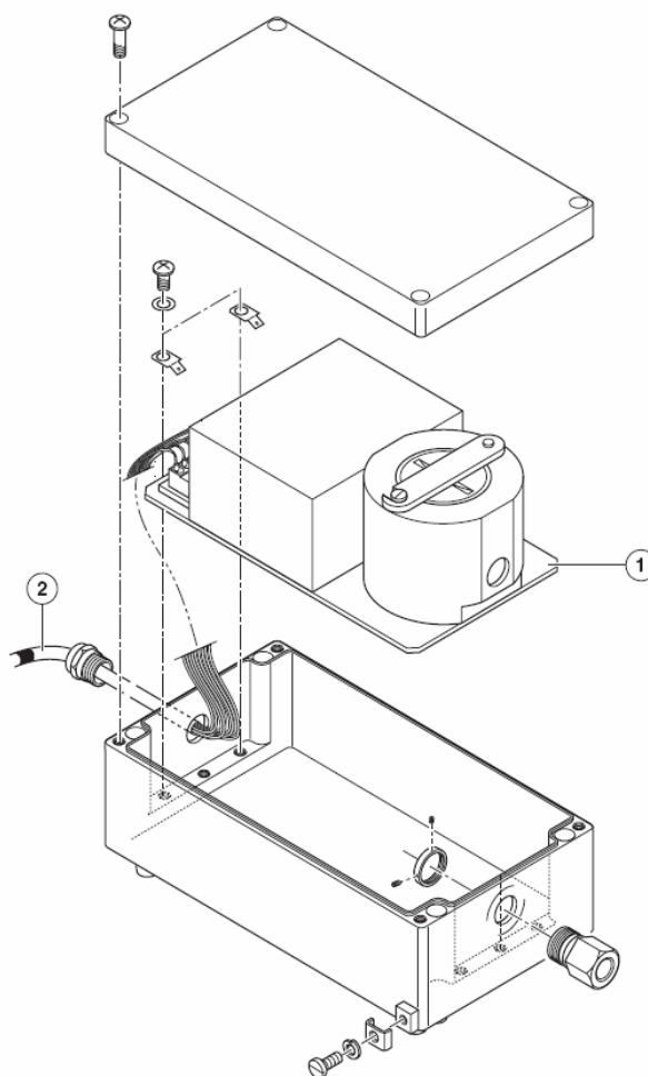
PSUx 120V Version
