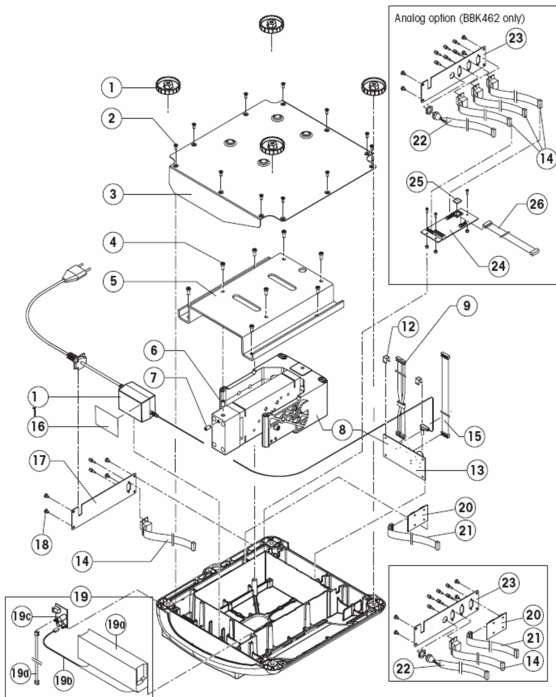
BBK4x2 Large Platform - Interior
