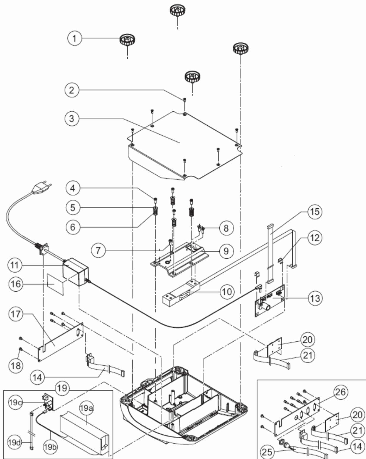
BBA422 Small Platform - Interior
