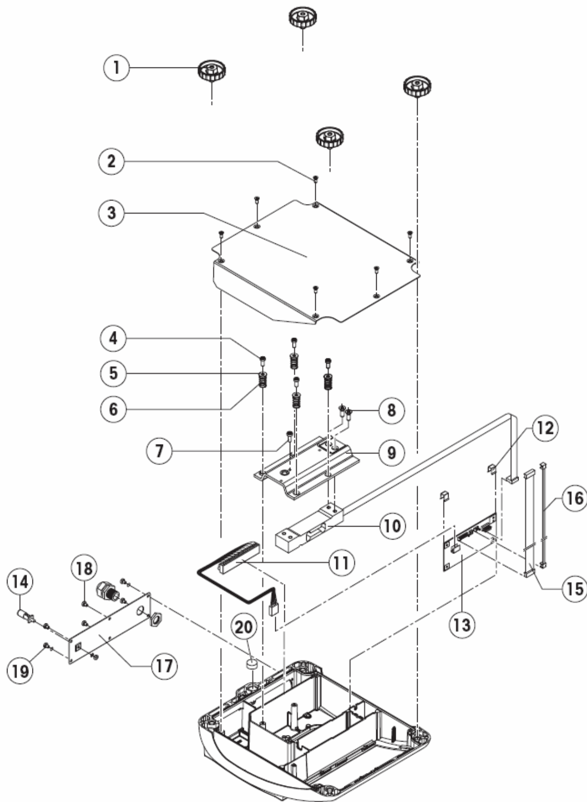
Viper EX - Small Platform Internal View
