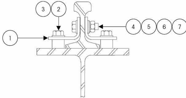
Anti Creep Angle Assembly
