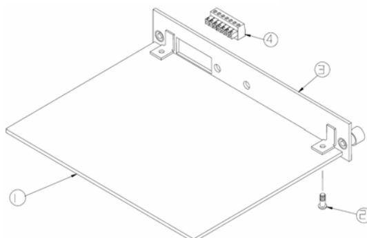
Analog PCB Assembly
