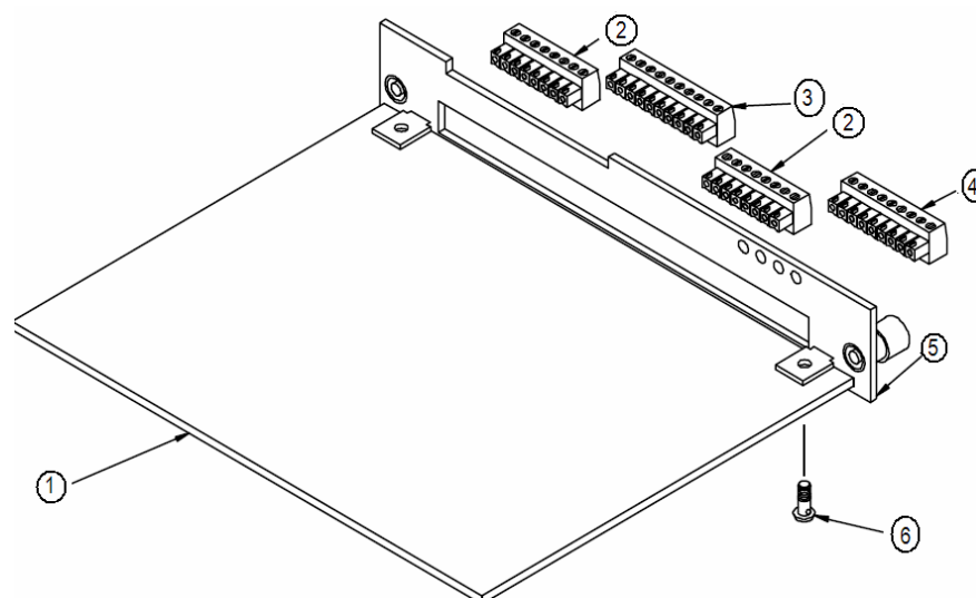
Multifunction PCB Assembly
