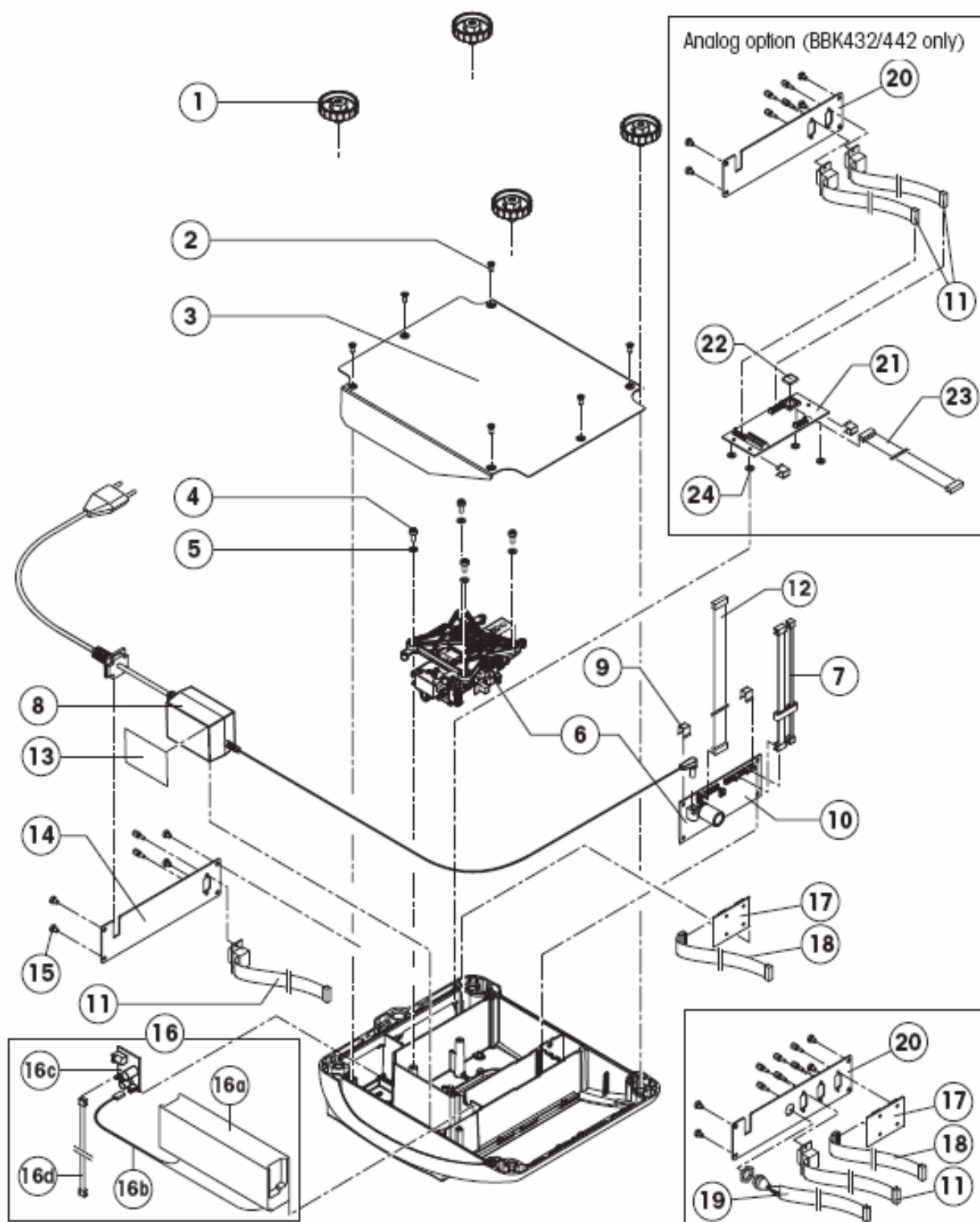
BBK4x2 Small Platform - Interior
