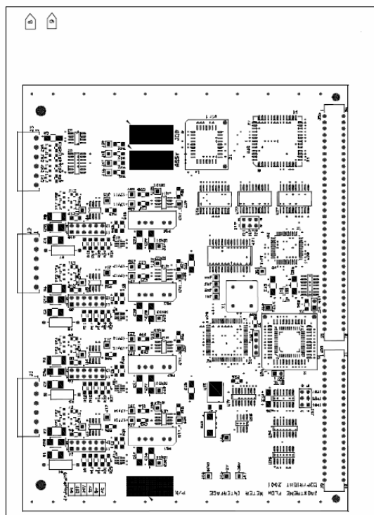
Flow Meter Interface Board
