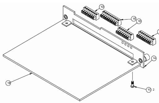
Multifunction PCB
