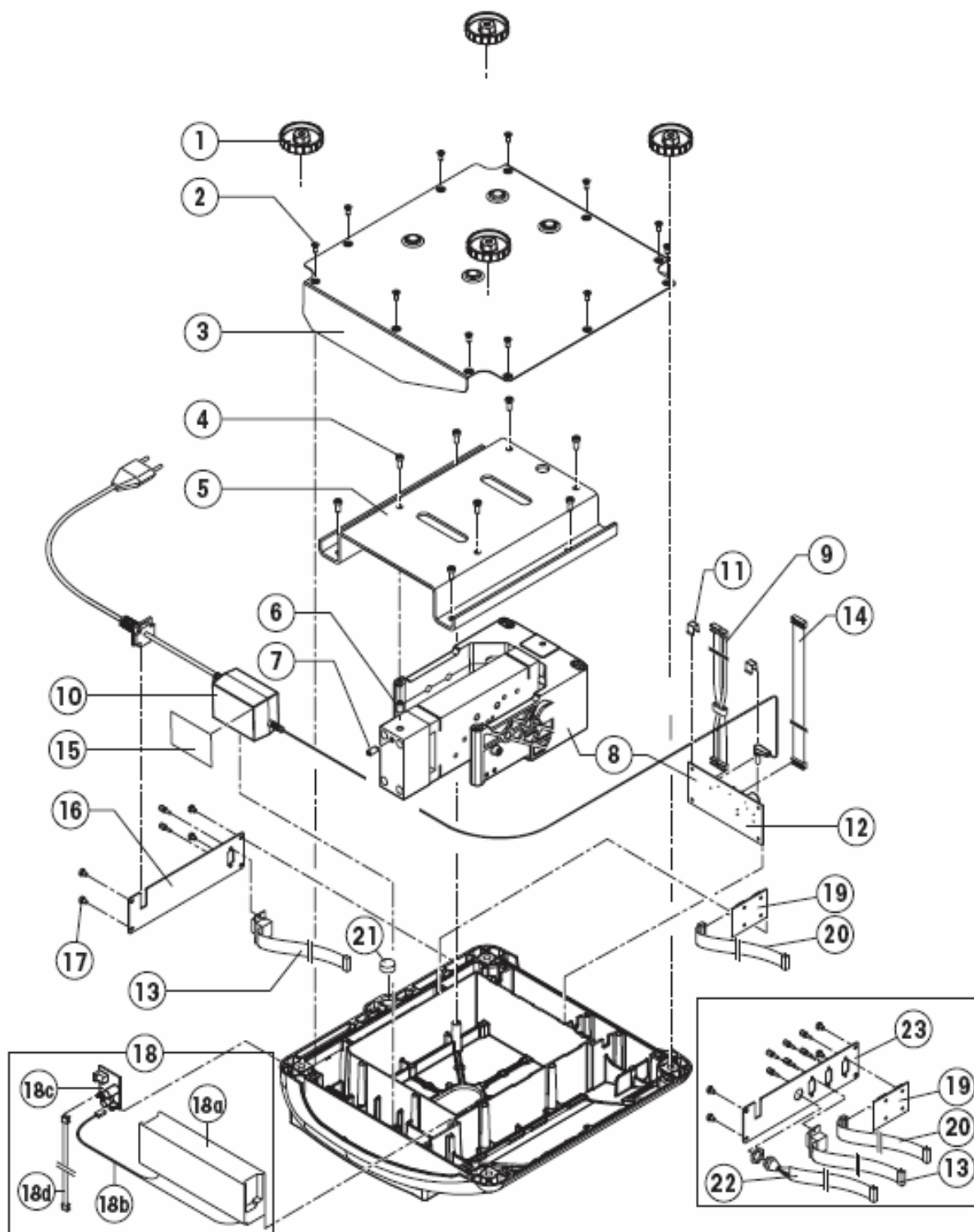
Viper - Large Platform MonoBloc Interior
