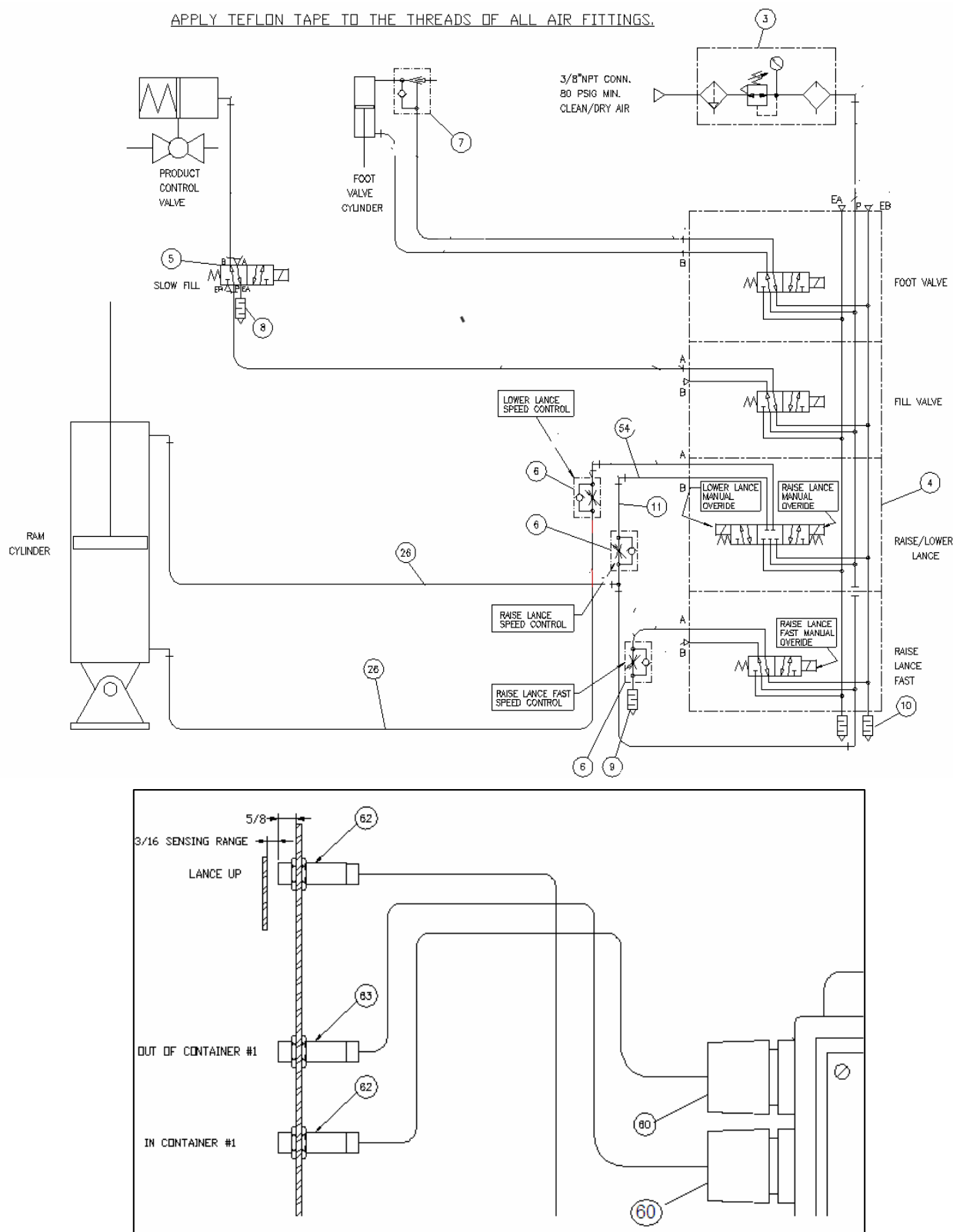
9127 Air Control Panel
