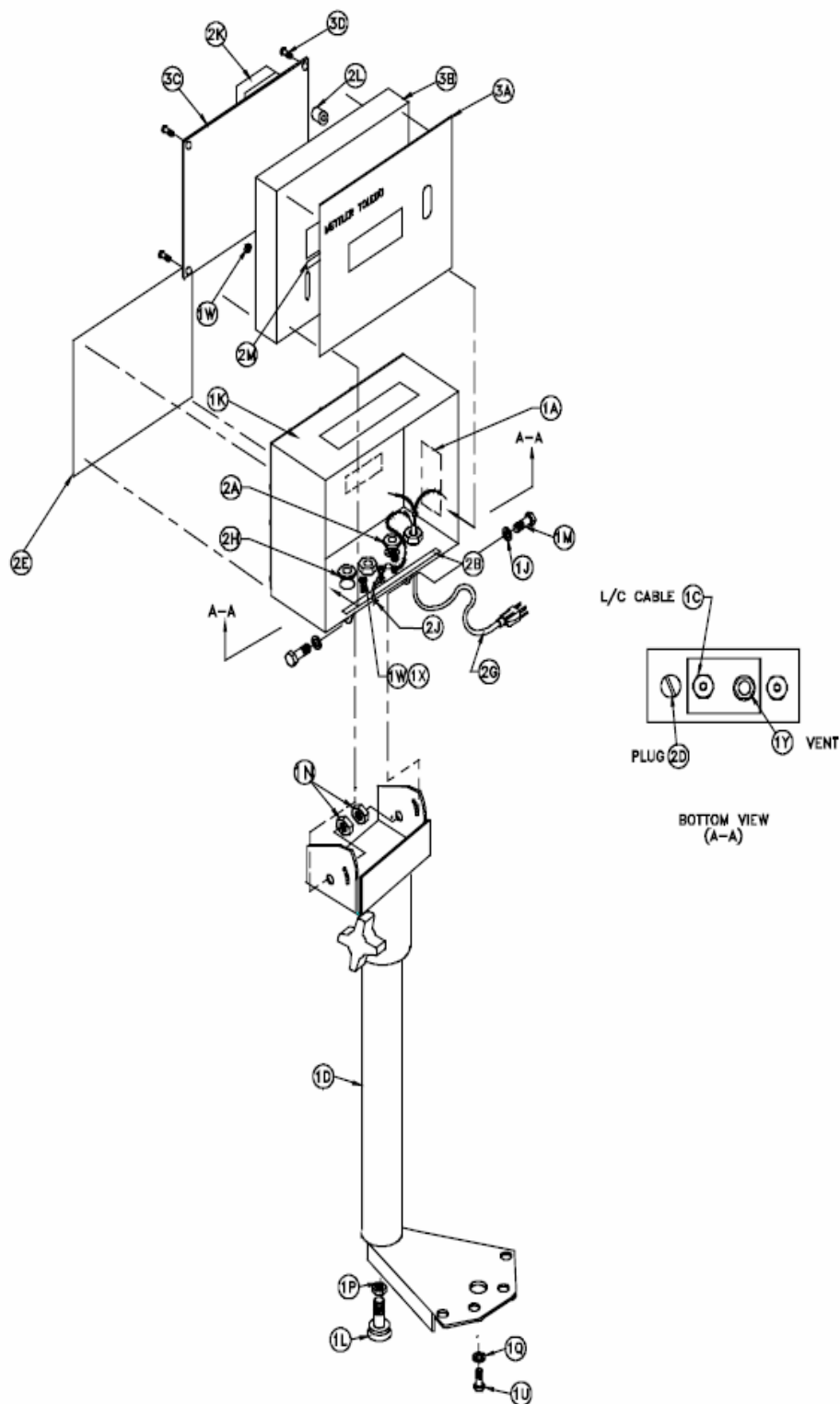
Speedweigh/Speedweigh Plus - Indicator/Column
