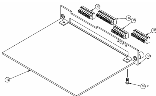
Multifunction PCB
