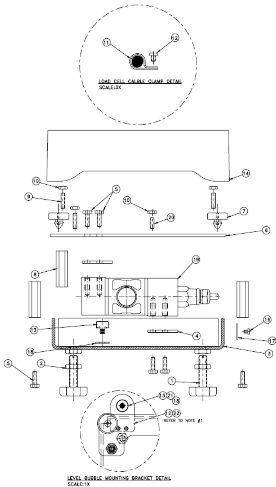
Trimweigh III - 9" Base
