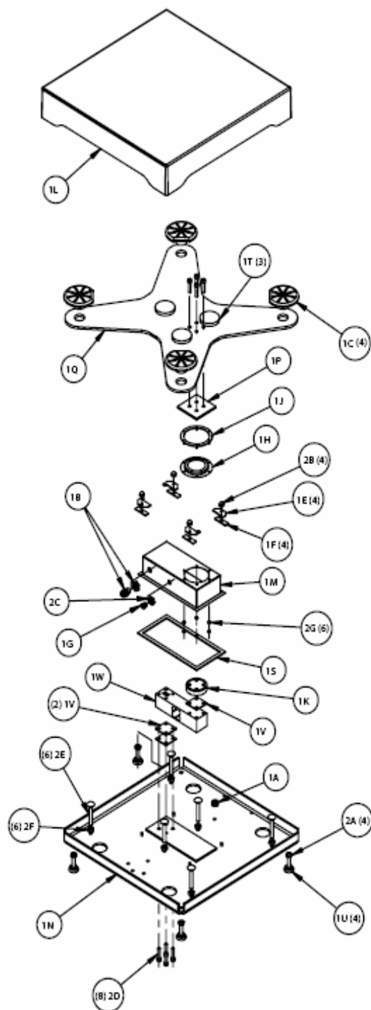
Speedweigh/Speedweigh Plus - Large Base
