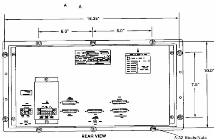
9215 Panel Mount
