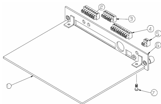
Controller PCB Assembly
