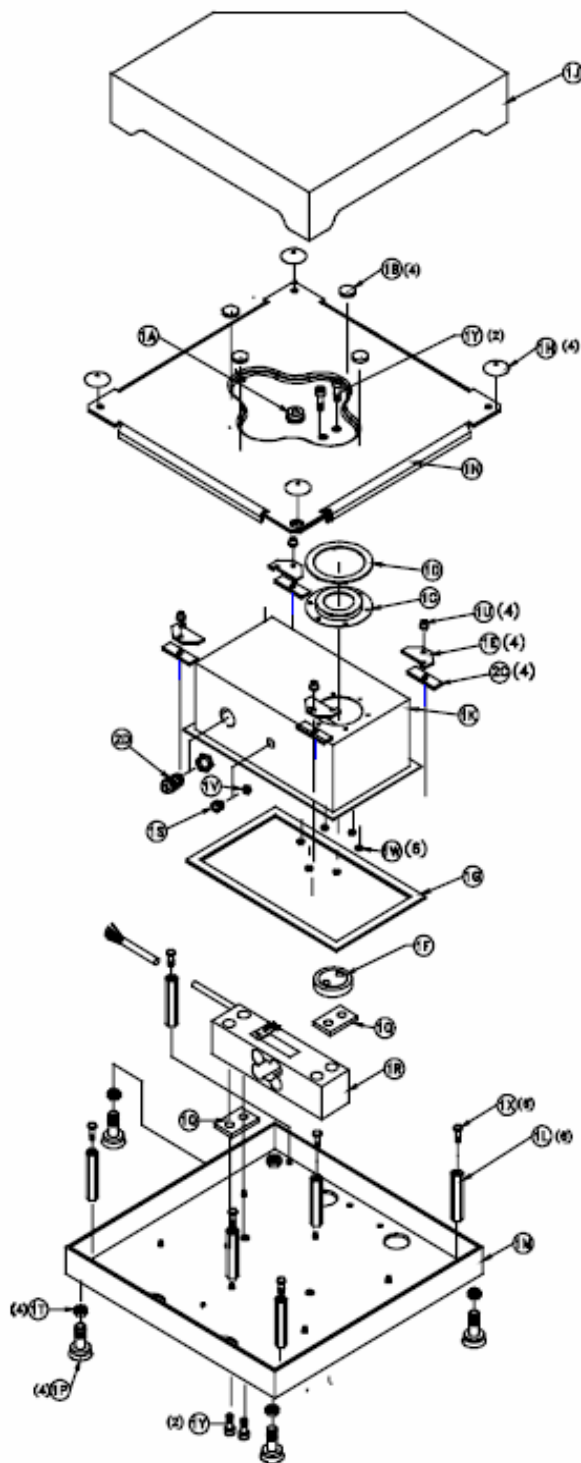
Speedweigh/Speedweigh Plus - Medium Base
