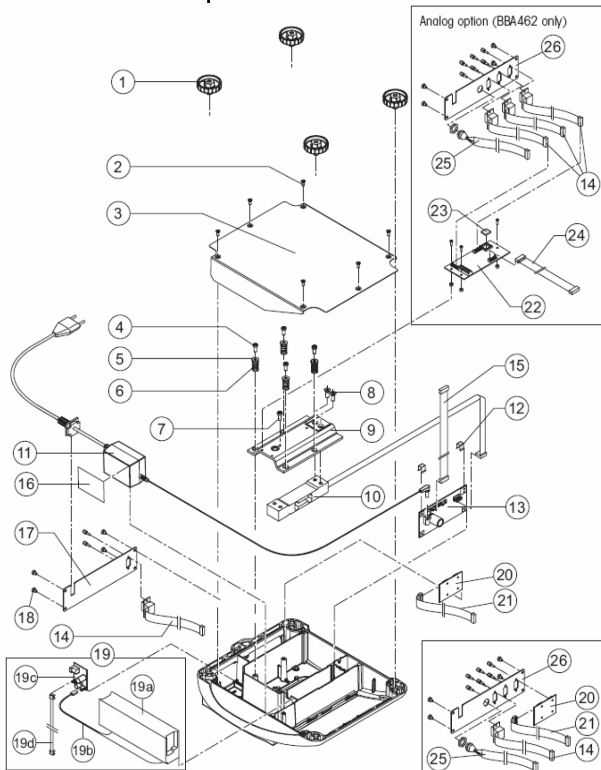
BBA4x2 Small Platform - Interior
