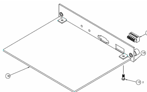
PROFIBUS I/F Assembly
