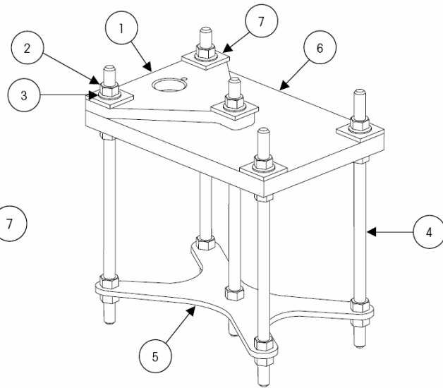
Standard Foundation Steel
