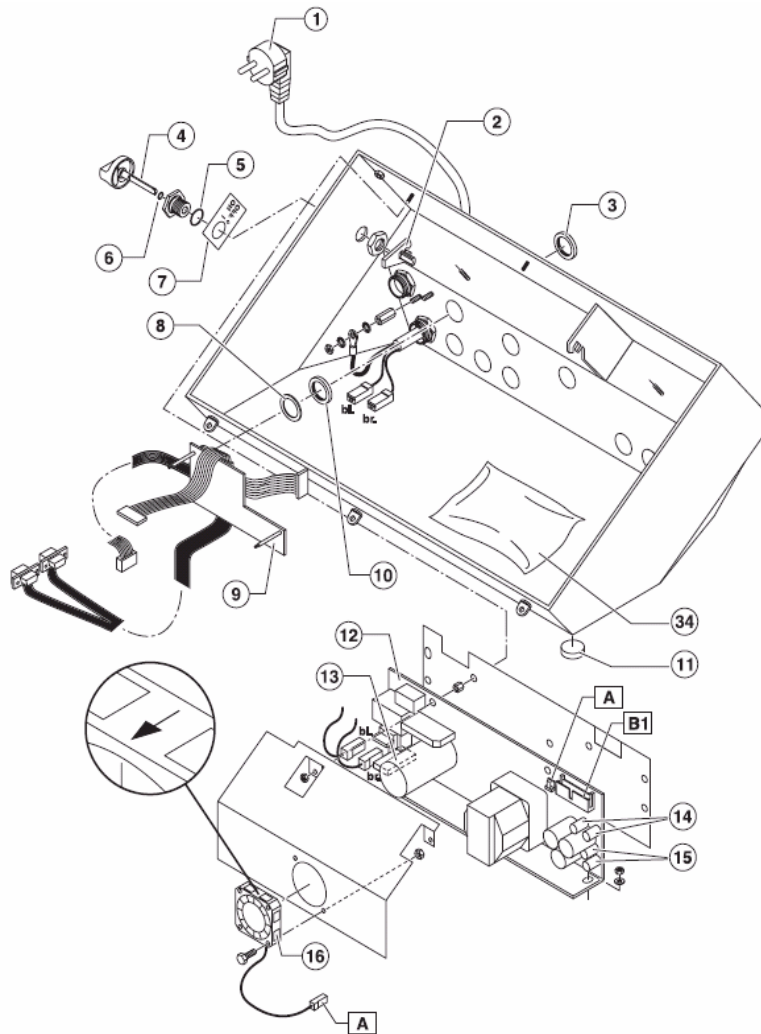
Housing and Power Supply Unit
