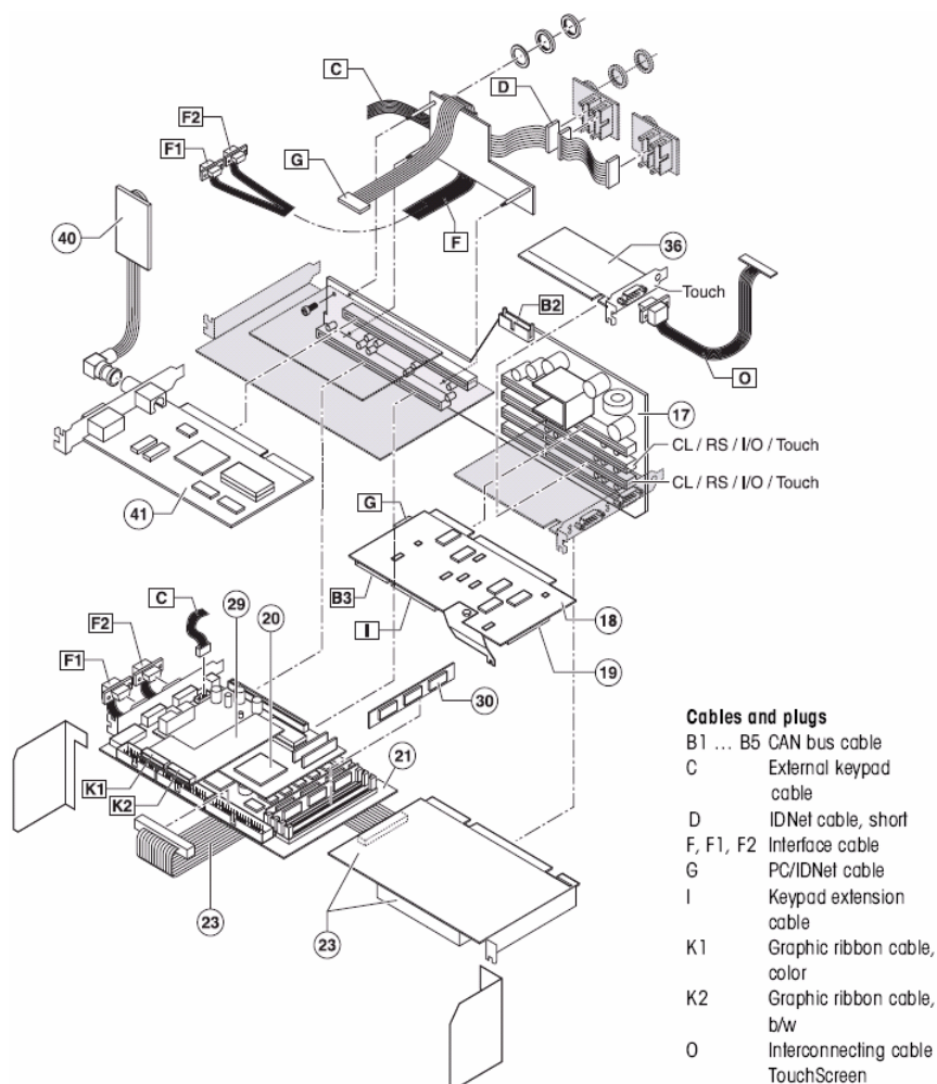
Electronics - Devices up to # 2178093
