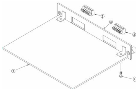
Dual Analog Output Assembly
