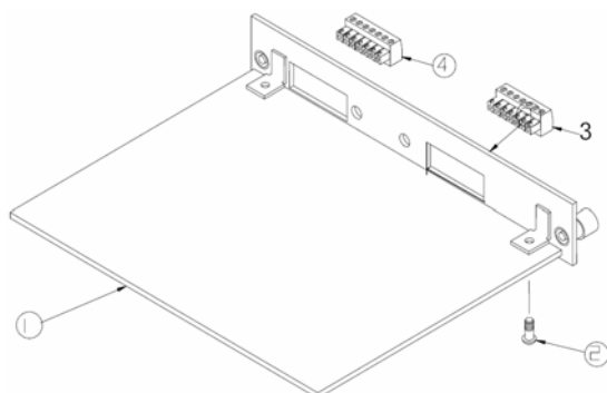
Dual Analog PCB Assembly
