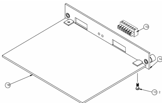
Powercell PCB
