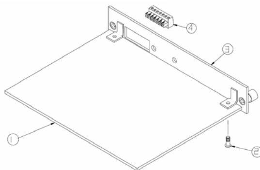
Analog Load Cell PCB Assembly
