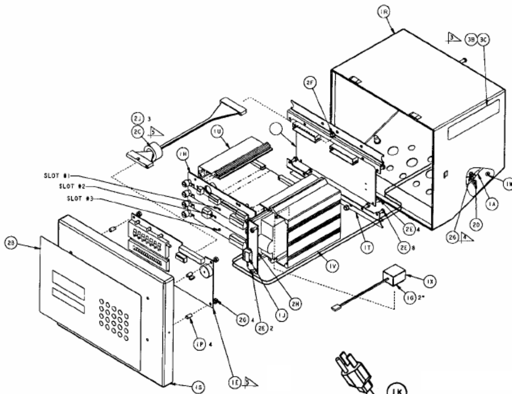
JagXtreme Harsh - Top/Front View
