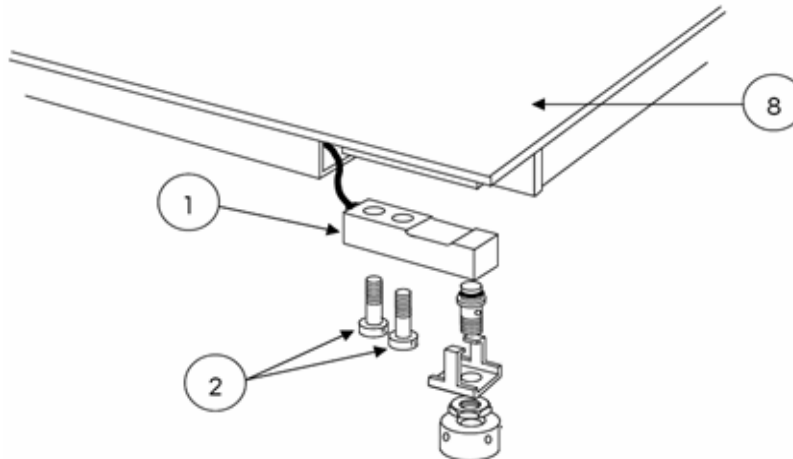
Load Cell and Level Foot Assembly Ver.1 (22561xxxxx)
