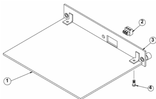
Allen-Bradley RIO Option
