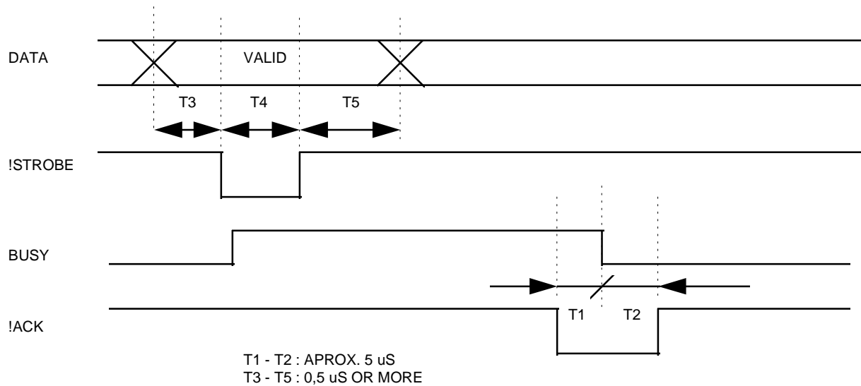
Fig. 2.3.3.2- Parallel input / output signal timing chart
