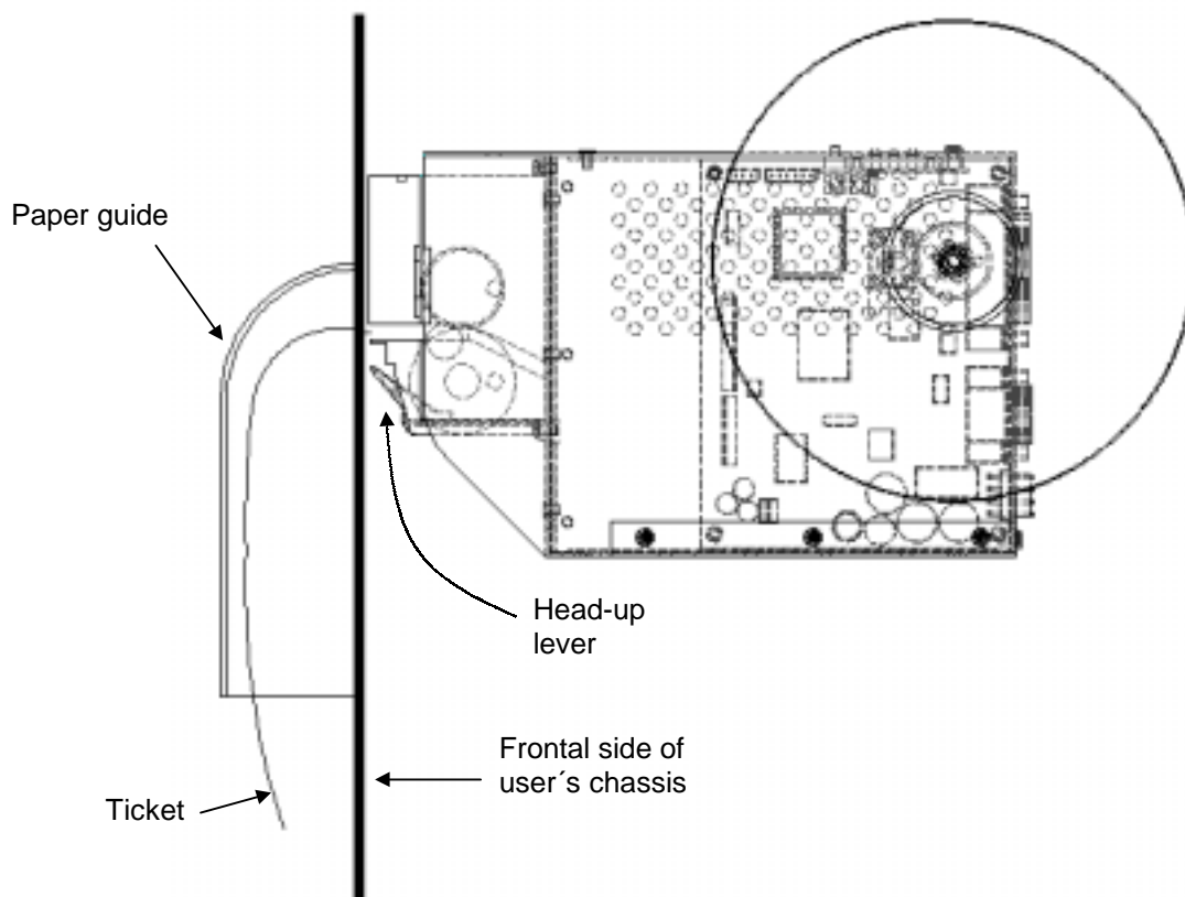
Fig. 2.2.2- Paper guide system.
