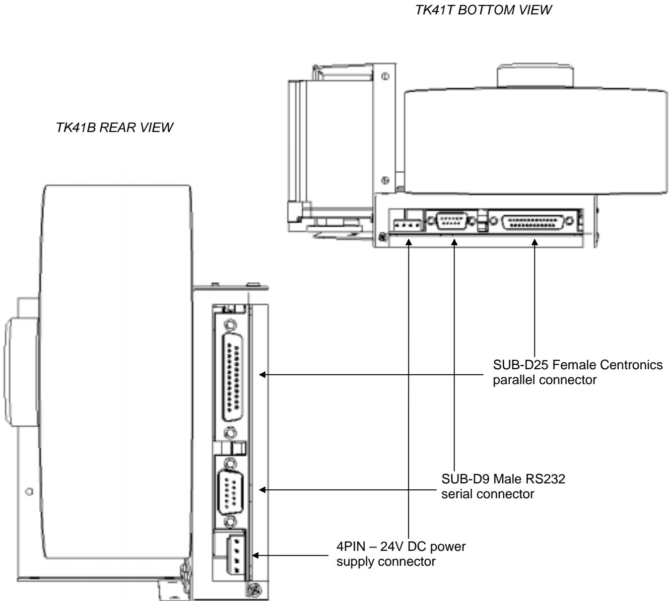
Fig. 2.3- TK41connectors location.
