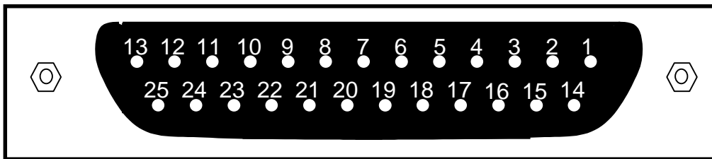
Fig. 2.3.3.1 – CENTRONICS connector as seen from outside the TK-41.
