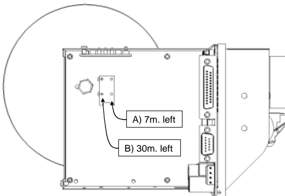
Fig. 2.2.0.C- Paper-near-end sensor positions.
