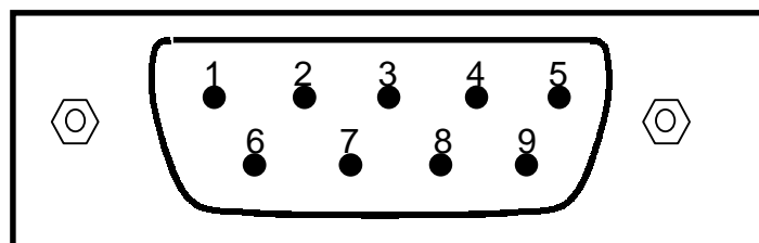
Fig. 2.3.2.1– RS-232 connector as seen from outside the TK41.
