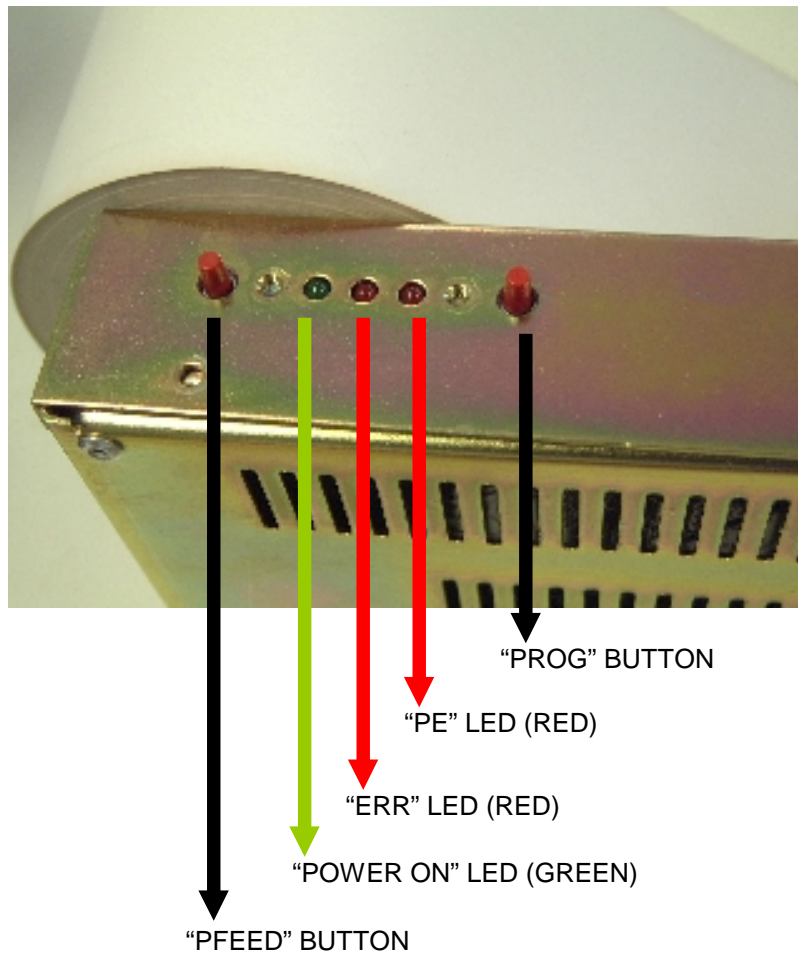
Fig. 3.3.1- TK41 Buttons & Leds identification.
