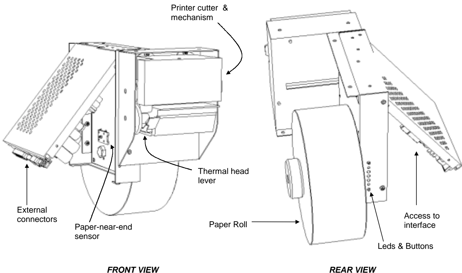
Fig. 2.2.0.A- Accessible parts of the TK41T.
