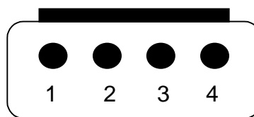
Fig.2.3.1- Power supply connector as seen from outside the TK41.
