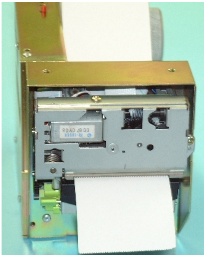
Fig.3.1.1- Automatic paper load sequence.
