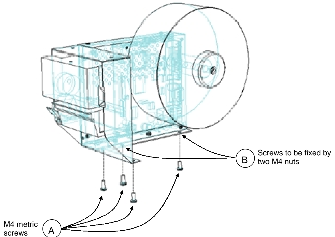
Fig. 2.1.2- Fixing the TK41B.
