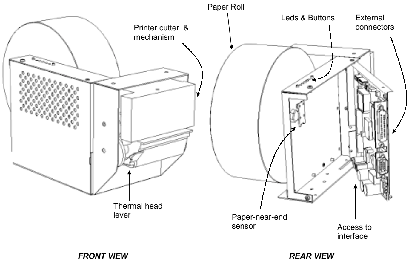
Fig. 2.2.0.B- Accessible parts of the TK41B.
