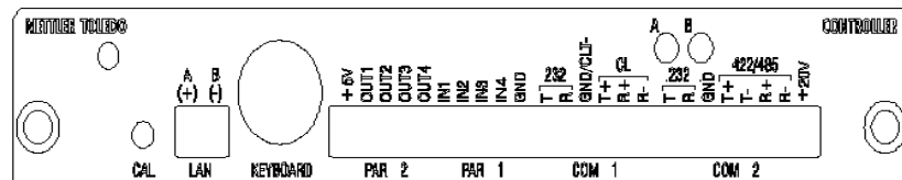
Figure 3-1: JAGUAR Terminal Controller PCB Rear View
