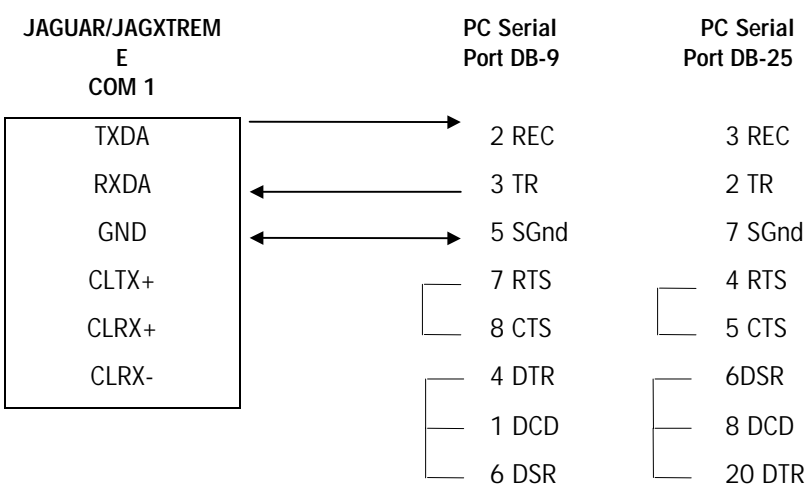
Figure 3-2: RS232 Connections to Terminal and PC Serial Port
