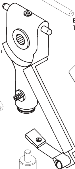
BB102A Upper Wheel Hanger - New Style (Complete with Tension Gauge Indicator, Spring & Cleaner Arm Assembly)
