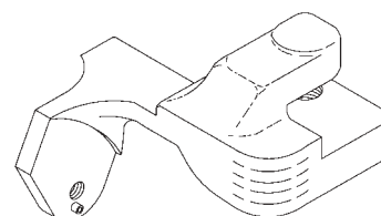
BB064-94 Rear Scraper Mount
