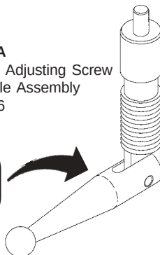
BB111 Wheel Adjusting Screw & Nut
