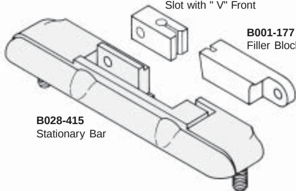
B002-119V Lower Saw Guide Slot with " V" Front
