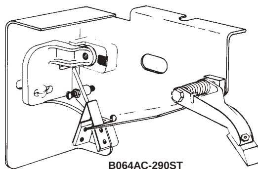
B064AC-290ST Cleaning Unit Assembly, Complete with Carbide Block
