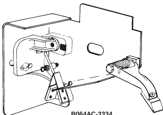
B064AC-3334 Cleaning Unit Assembly, Complete with Carbide Block
