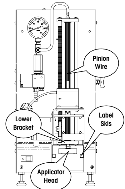
Model 317 Applicator Front View (Cover removed)
