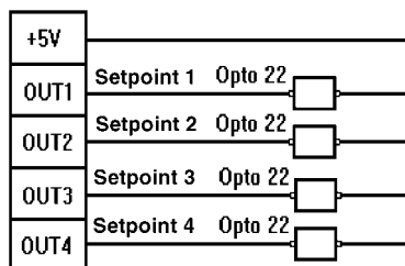
Figure 2-h: Output Wiring Example
