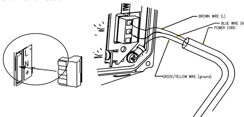
Power Connection for Wall/Desk Mount Terminal
