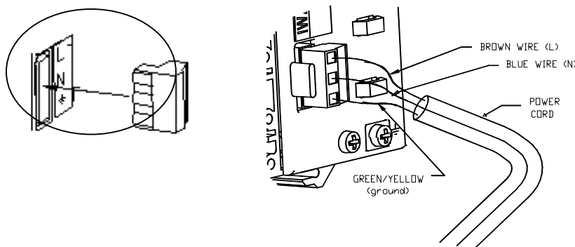
Power Connections for Panel Mount Terminal
