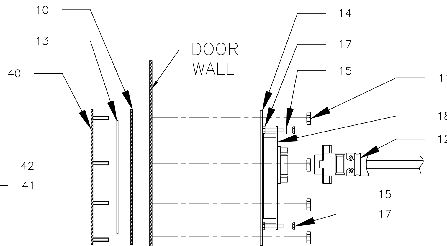
SECTION A-A EXPLODED VIEW
