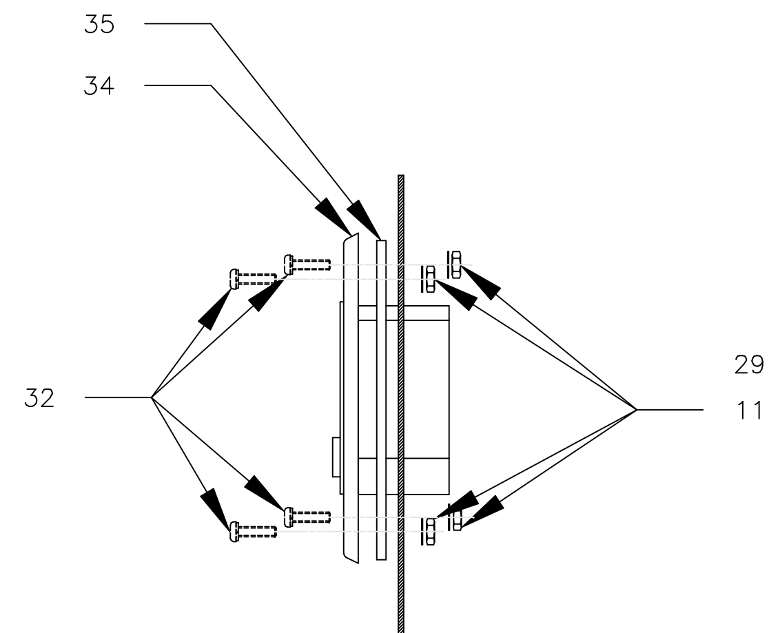
SECTION B-B EXPLODED VIEW
