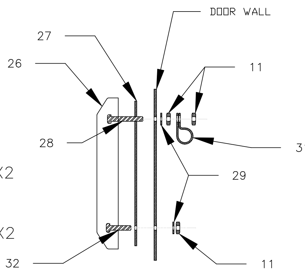
SECTION C-C EXPLODED VIEW
