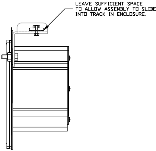
DETAIL A – EXPLODED VIEW OF IND560 MOUNTING
