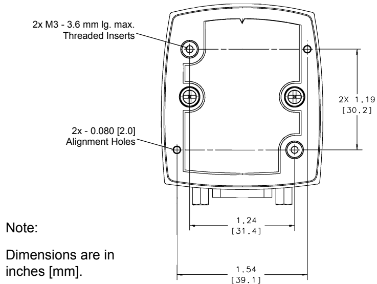
Figure 2-3. MS 804FZY/MS 904HS Mounting Dimensions
