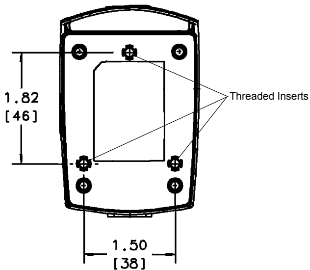
Figure 2-2. MS 3204 Mounting Dimensions
