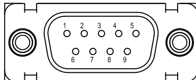
Figure 7-1. MS 3204 Connector
