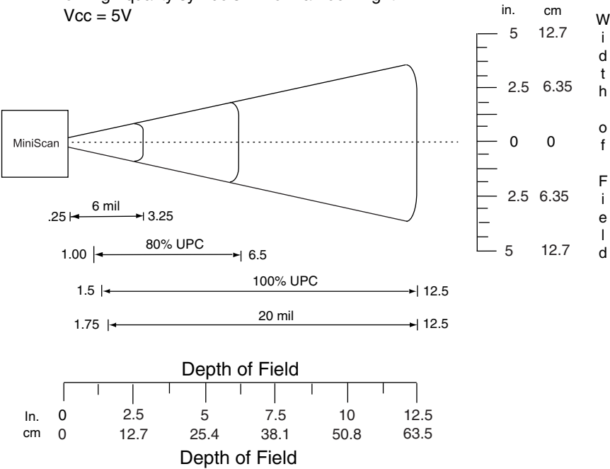
Figure 7-5. MS 3204 Omnidirectional Decode Zone
