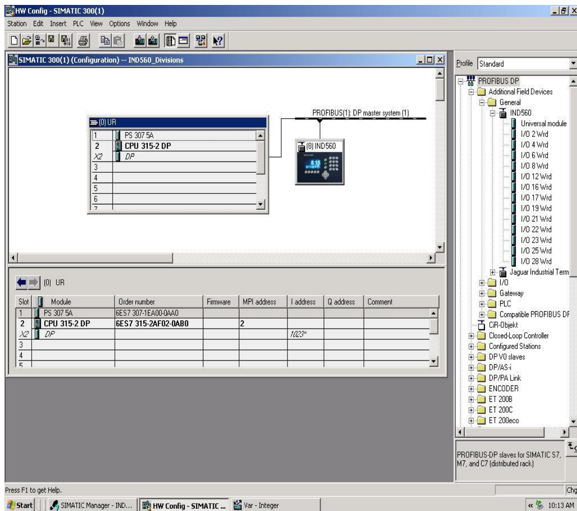
Figure 4-5: Hardware Setup
