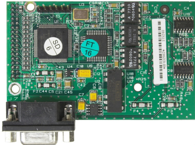
Figure 4-2: PROFIBUS Kit Option Board, Panel Mount Version
