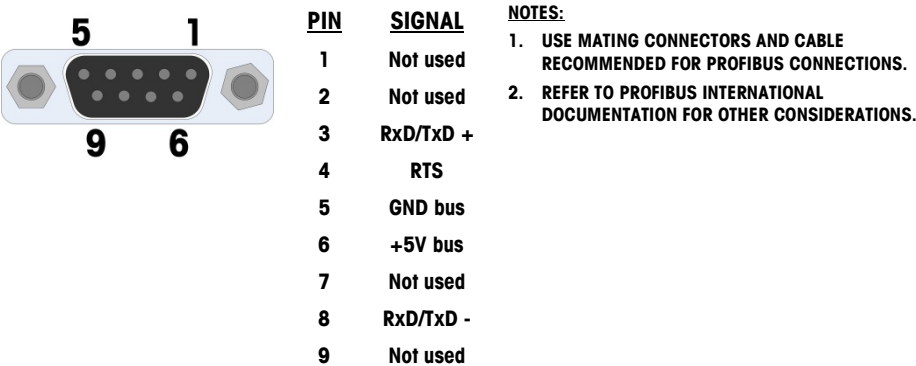
Figure 4-3: PROFIBUS Option Card DB-9 Connector
