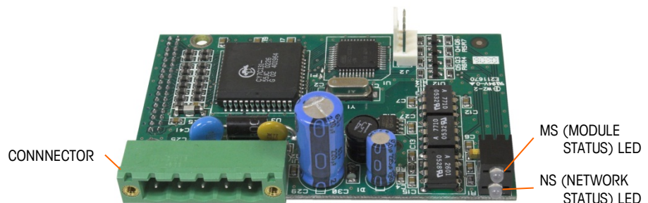
Figure 3-2: DeviceNet Option Board Components
