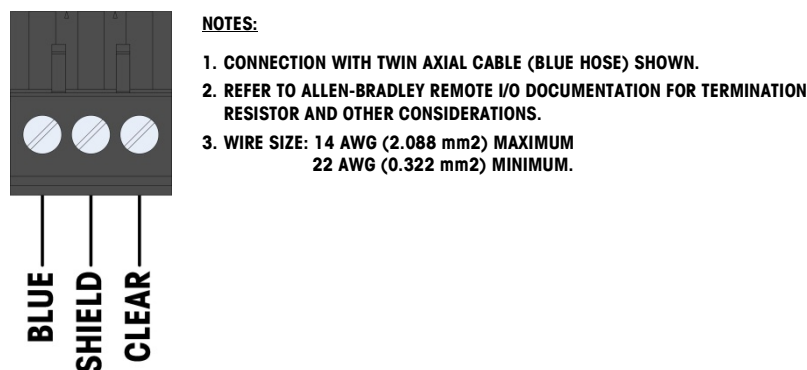
Figure 2-2: Three-Position Terminal Strip Wiring
