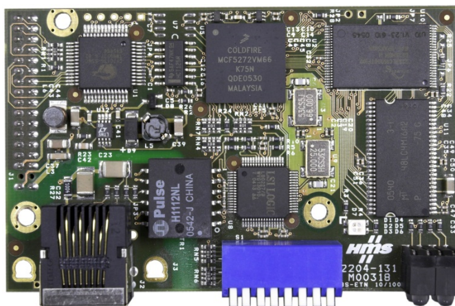
Figure 5-1: EtherNet/IP Module
