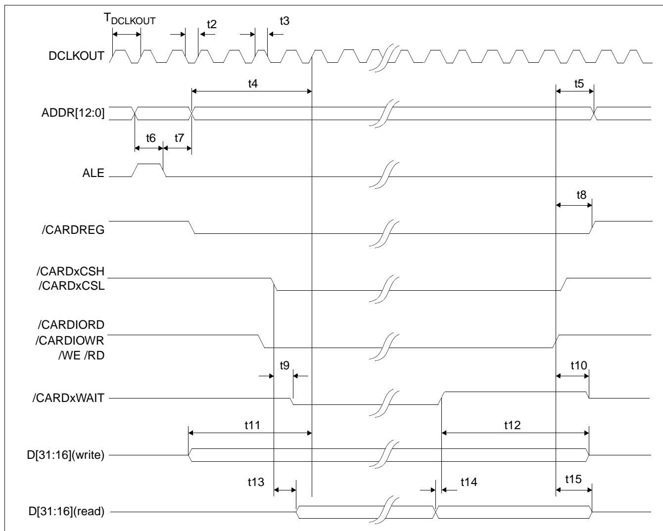
Figure 7-9: Philips Timing
