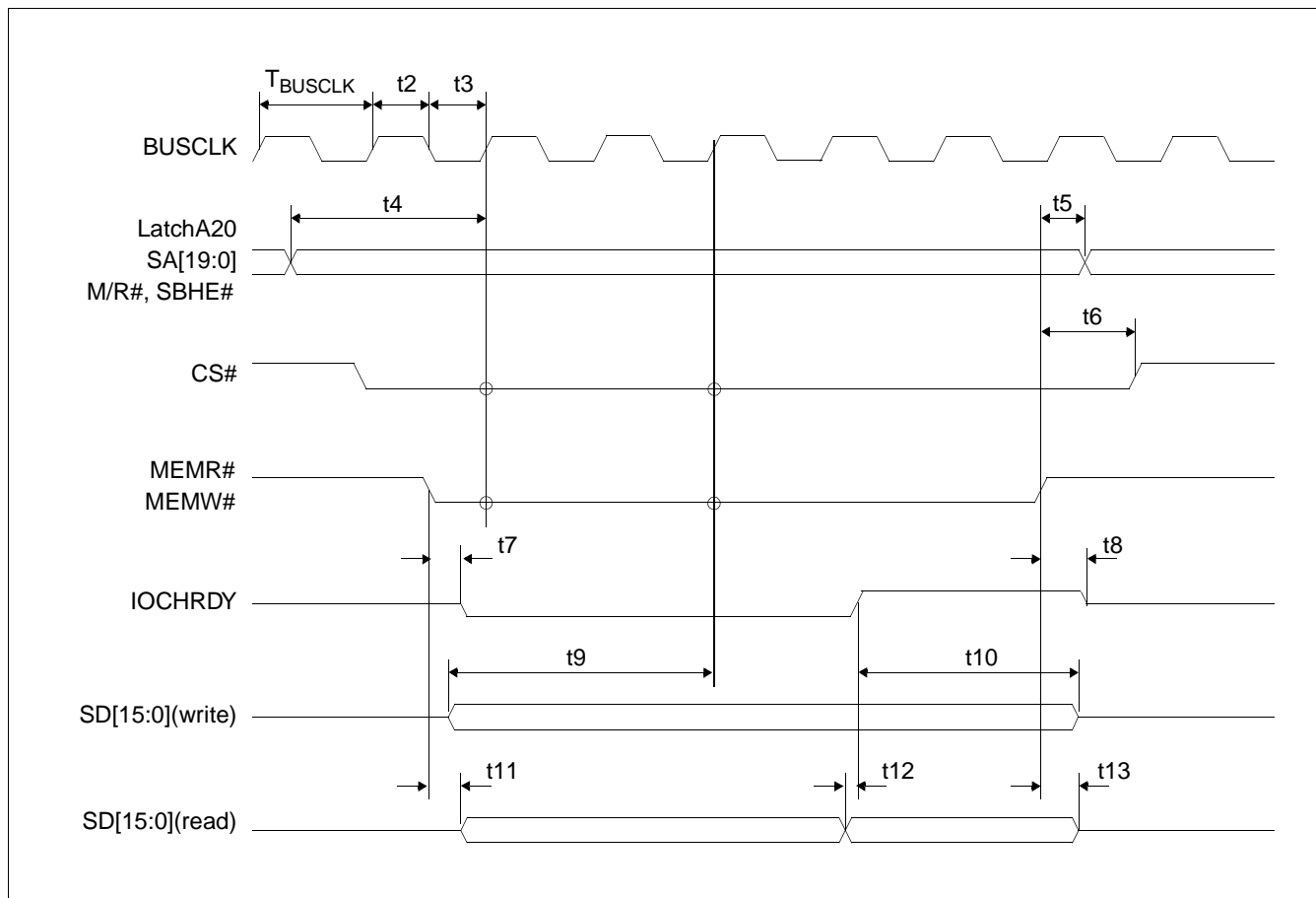
Figure 7-4: MIPS/ISA Timing
