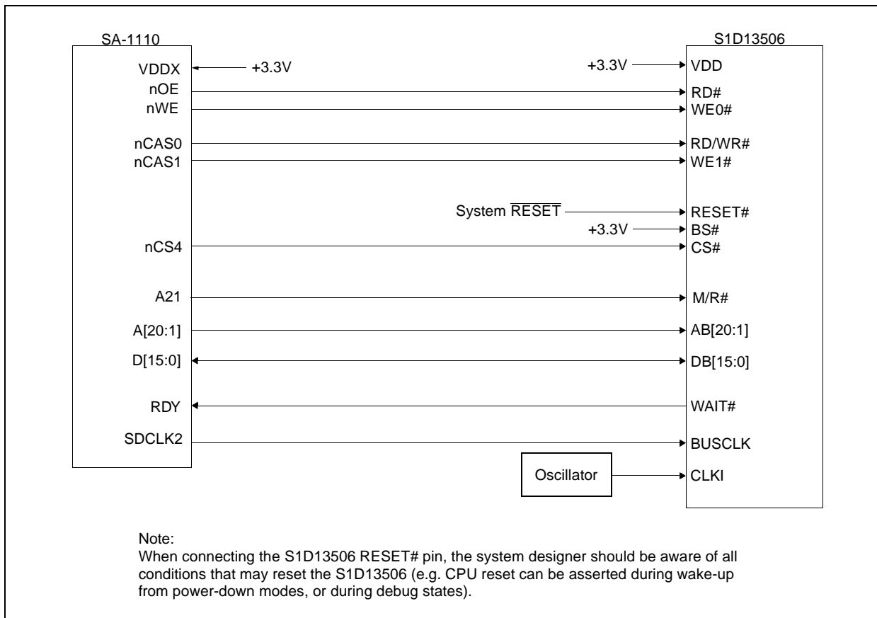
Figure 4-1: Typical Implementation of SA-1110 to S1D13506 Interface
