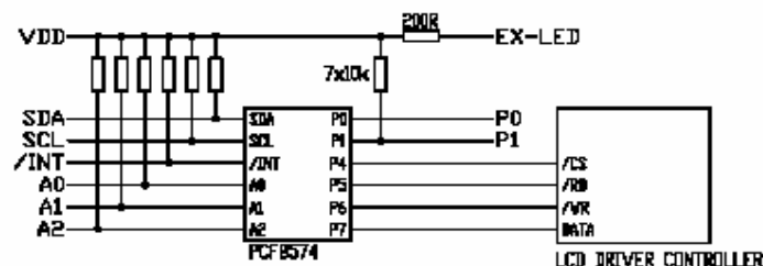
Interface Circuit Scale=free
