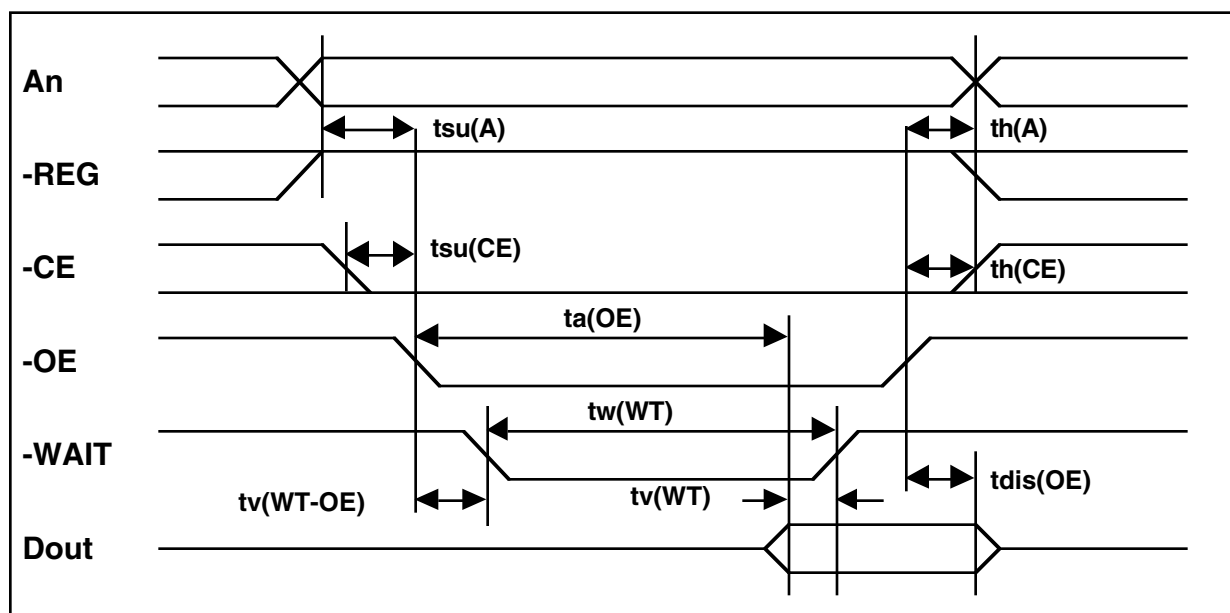
Figure 4-3 Common Memory Read Timing Diagram
