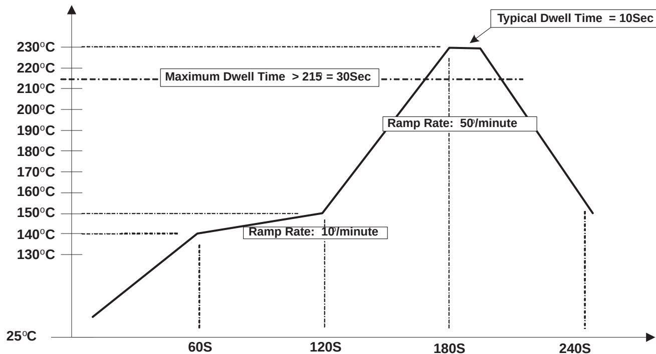
Figure 13 IR Reflow Ramp Rate Requirements
