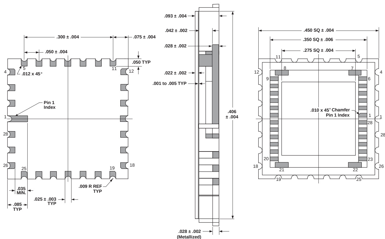
Figure 11 OV7640/OV7141 Plastic Package Specifications
