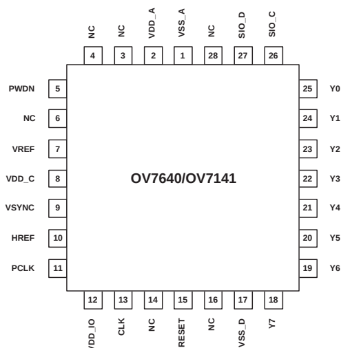
Figure 1 OV7640/OV7141 Pin Diagram
