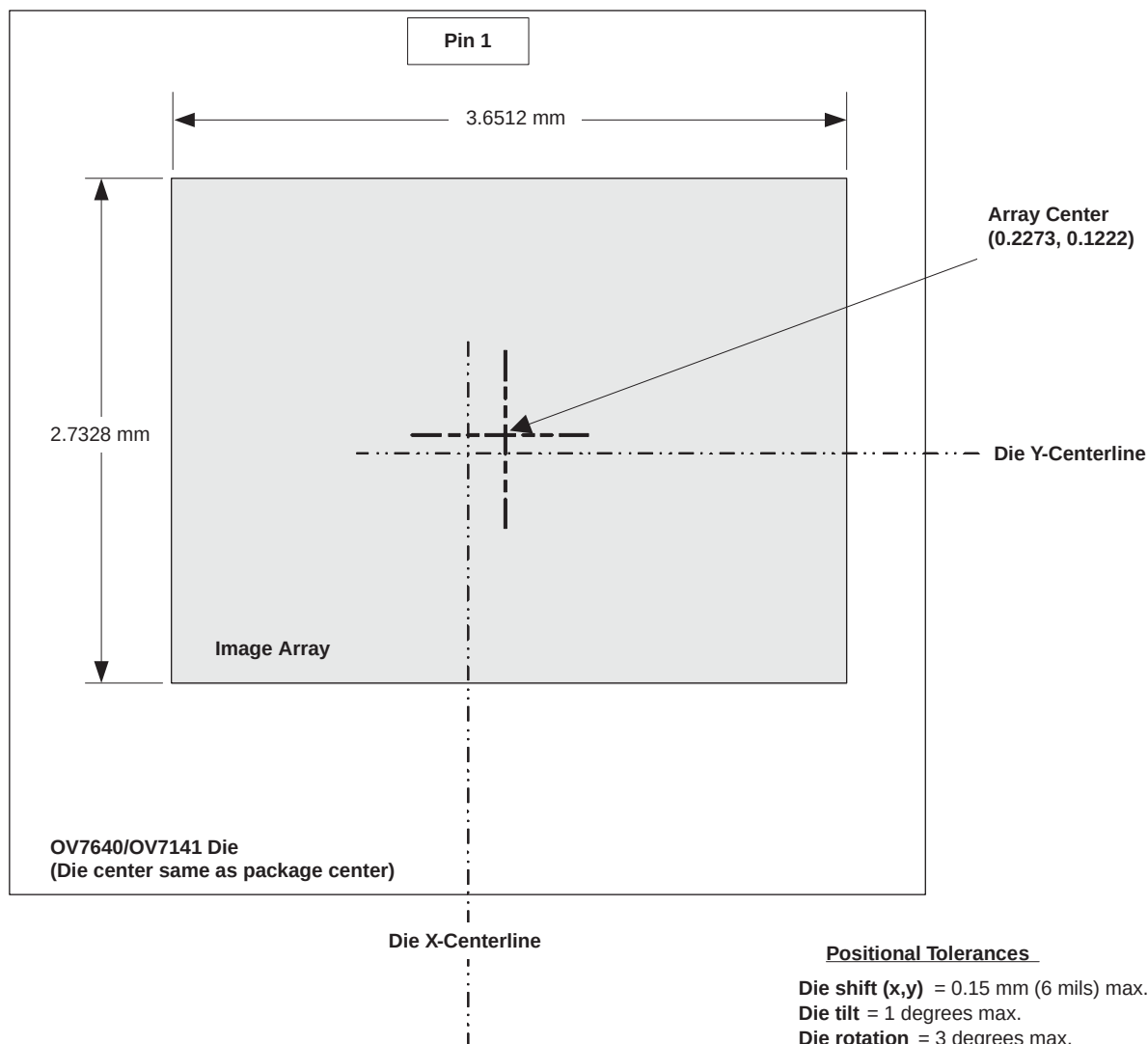
Figure 12 OV7640/OV7141 Sensor Array Center
