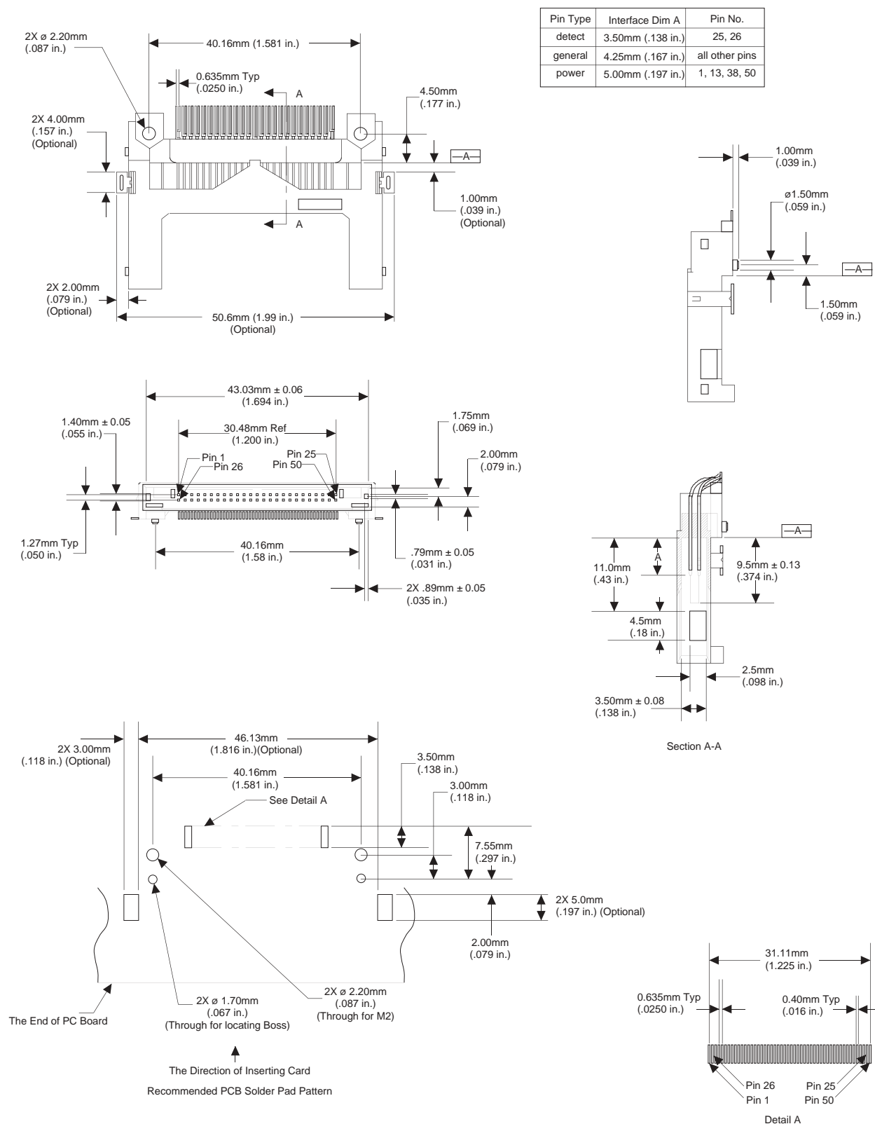
Figure 7 Surface Mount Right Angle CF Card Slot Header
