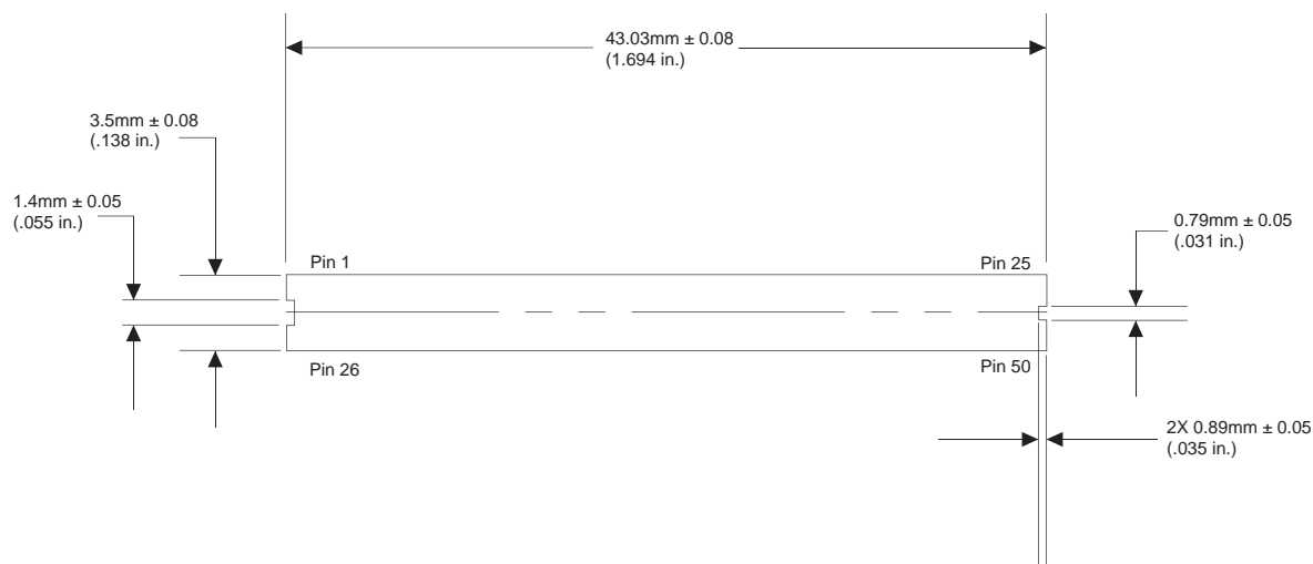
Figure 4 Pin Connector Opening
