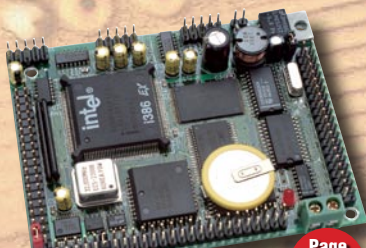
i386-Engine-L (IEL)
