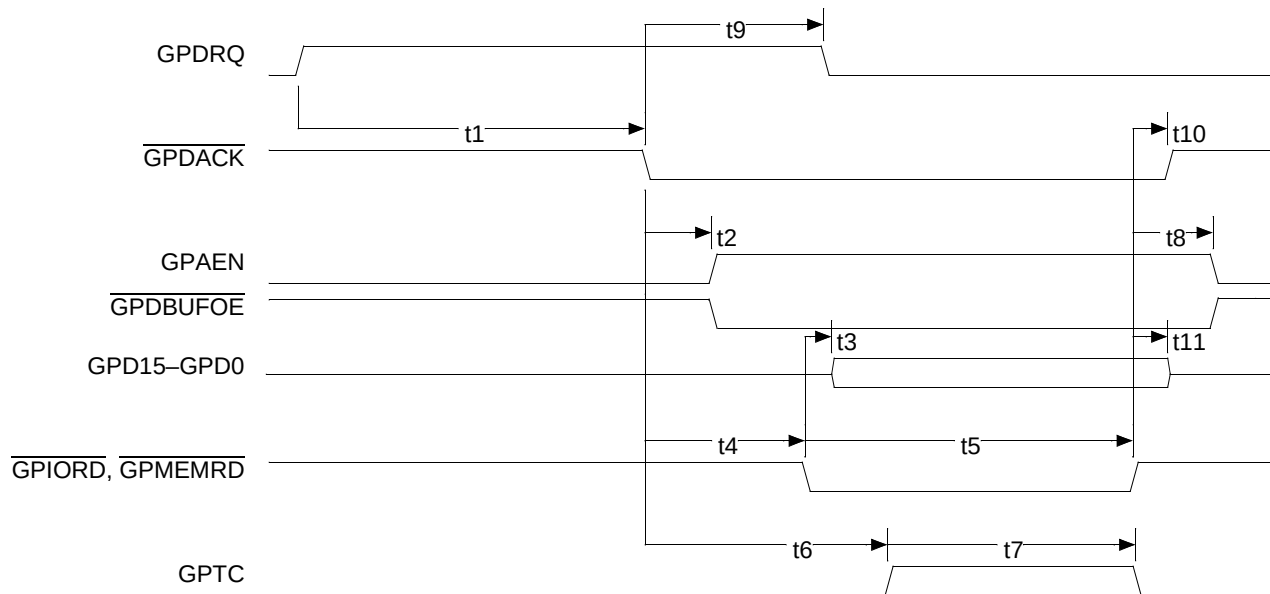
Figure 37. GP-DMA Write Cycle Timing
