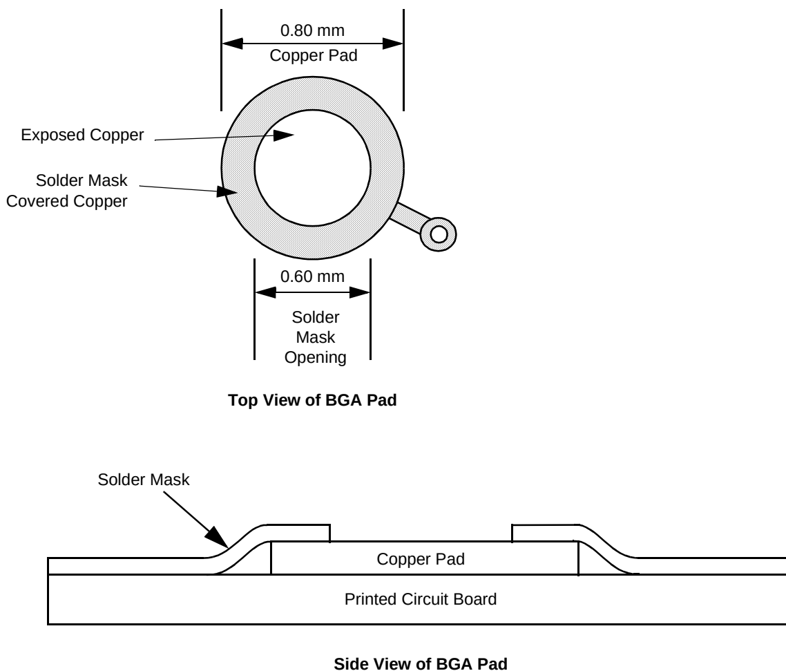
Figure 40. BGA Ball Pad Layout
