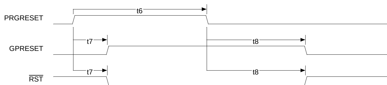
Figure 29. PRGRESET Timing
