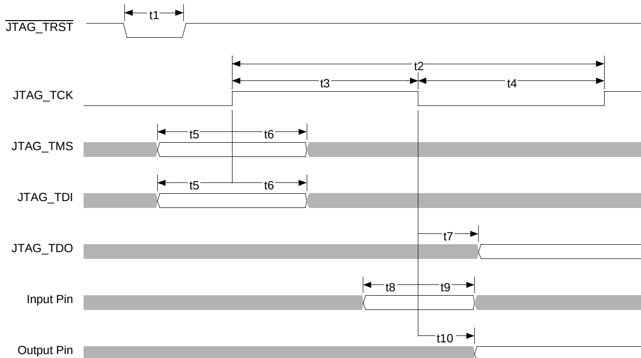
Figure 39. JTAG Boundary Scan Timing
