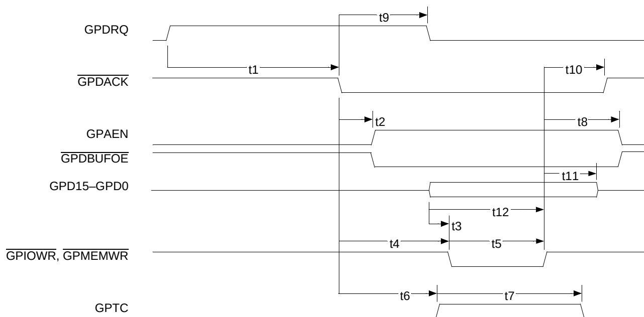
Figure 36. GP-DMA Read Cycle Timing
