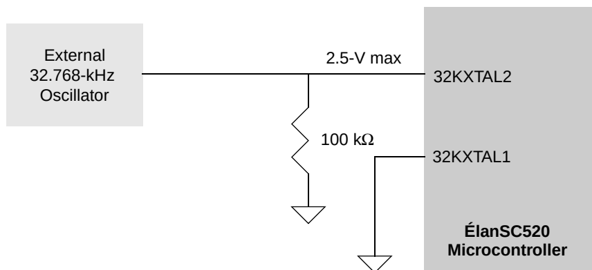
Figure 10. Bypassing the 32.768-kHz Oscillator
