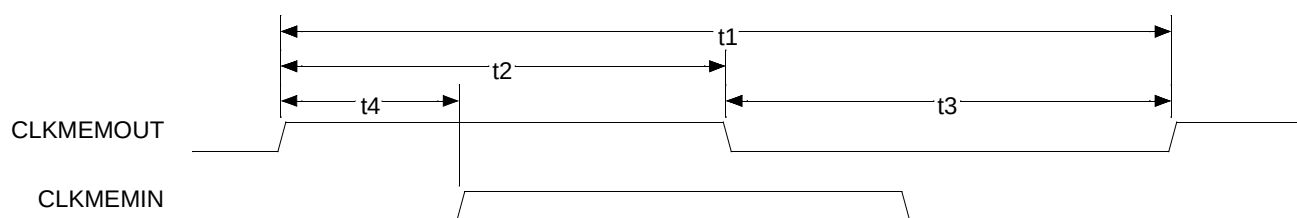
Figure 34. SDRAM Clock Timing
