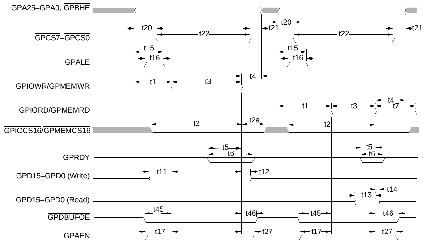
Figure 35. GP Bus Non-DMA Cycle Timing
