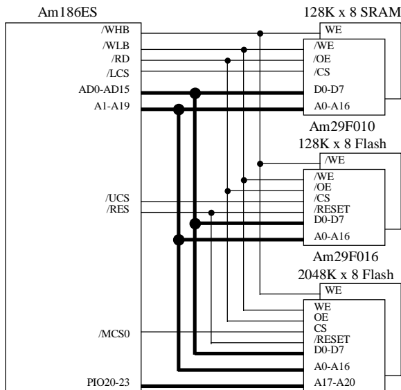
Figure 1. The Am186ES with extended Flash Memory
