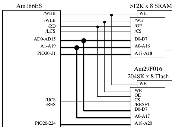
Figure 2. The Am186ES with extended single banked Flash and SRAM memory
