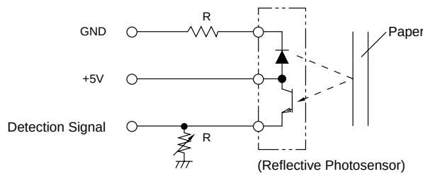
Fig. 2-15 Paper-Out Detector
