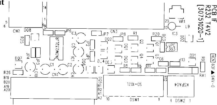
RS-232C Interface Board (Ver.2)
