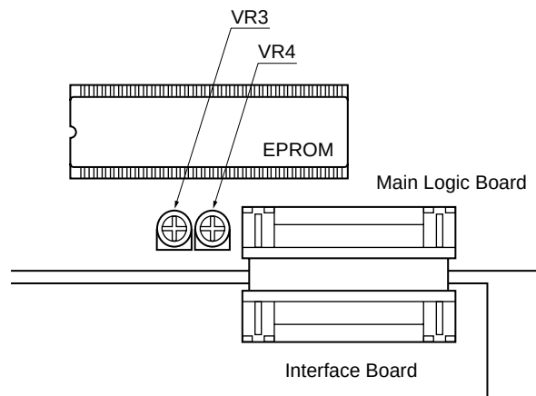
Fig. 1-6 Sensor Adjustment
