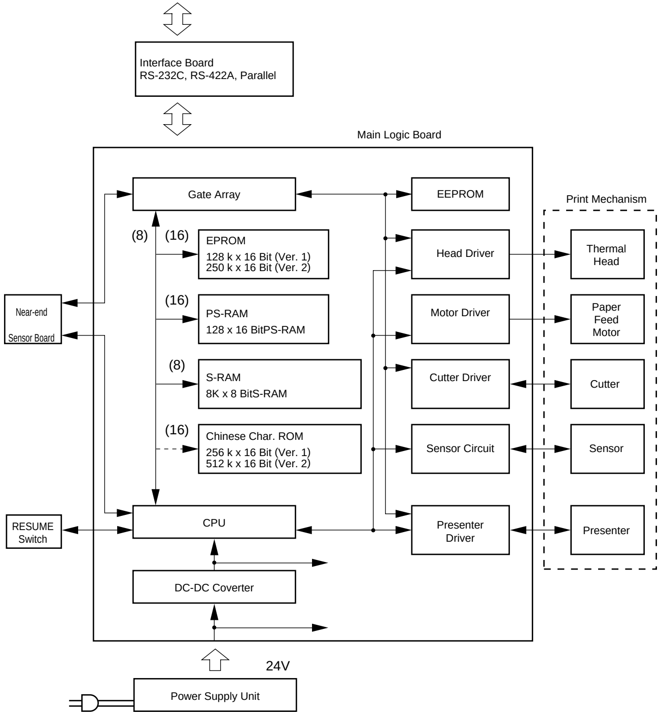
Fig. 2-1 Block Diagram
