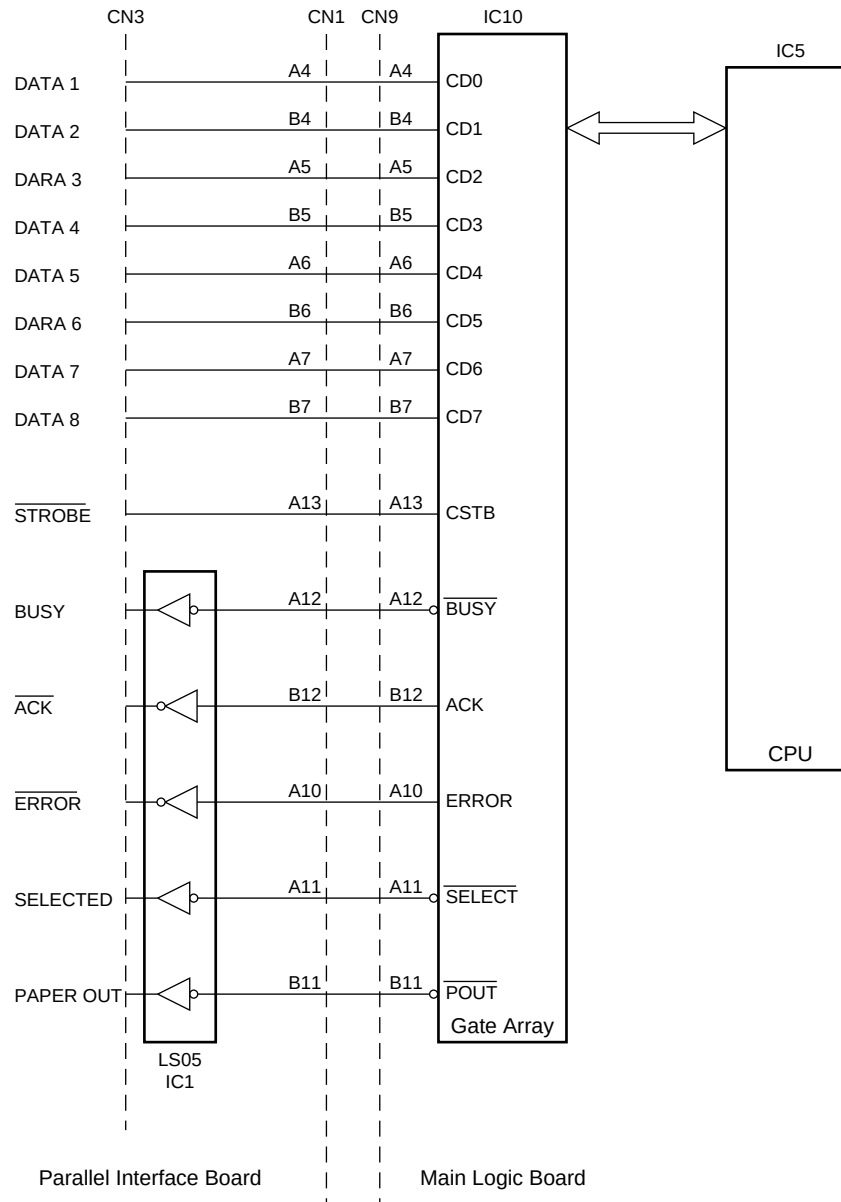
Fig. 2-4 Parallel Interface
