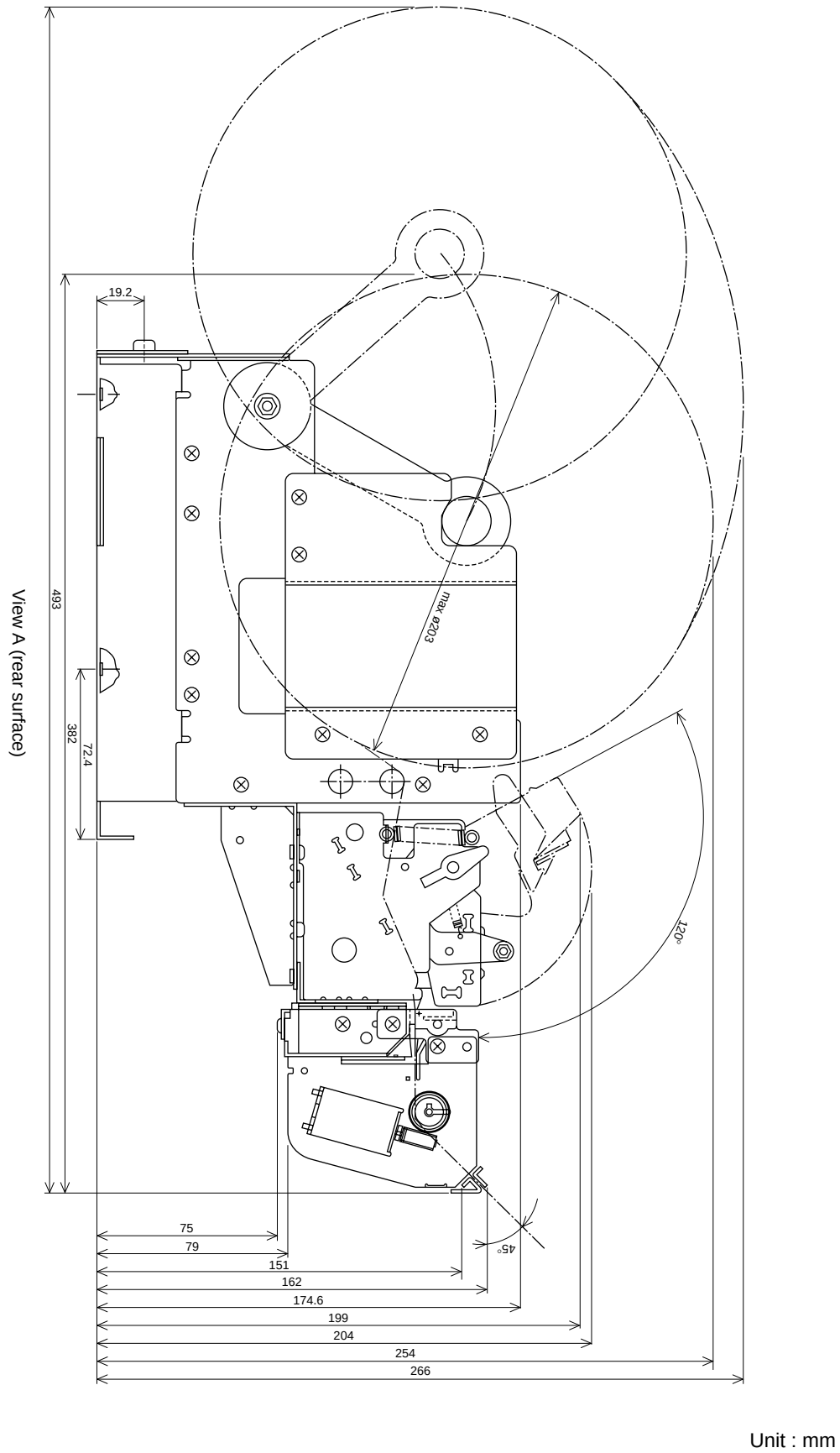
Fig. 1-1-c External Dimensions (TUP482)
