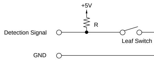
Fig. 2-18 Head-Up Detector
