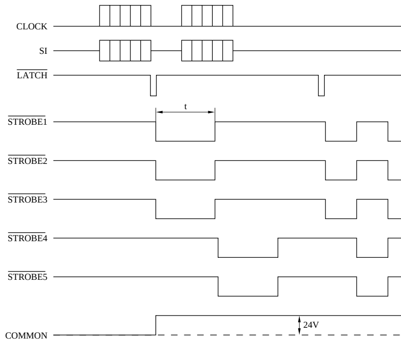
Fig.2-6 Timing Chart
