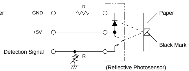
Fig. 2-16 Black-Mark Detector
