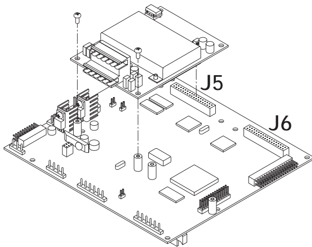
Figure 1. Installing Option Card Onto CPU Board
