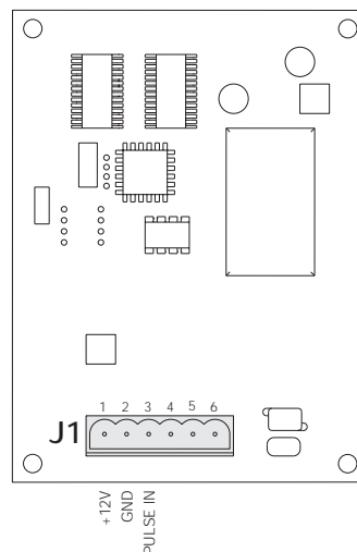
Figure 3. Pulse Input Card
