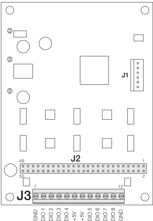
Figure 2. Digital I/O Expansion Card
