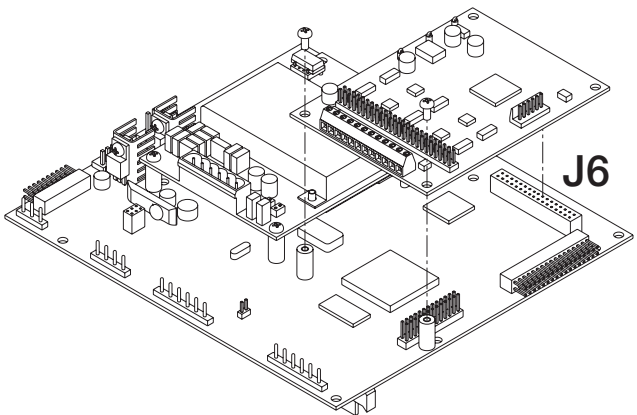
Figure 1. Installing Option Card Onto 920i CPU Board
