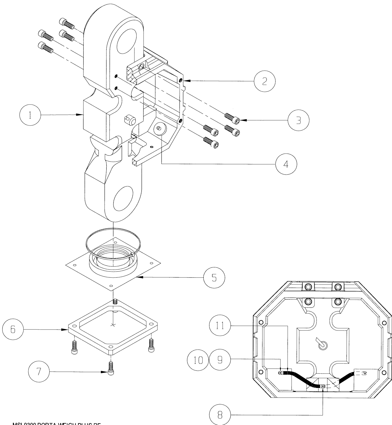
MSI-9300 PORTA-WEIGH PLUS RF MID-SECTION ASSEMBLY 50 & 70,000 LBS Measurement Systems International 14240 Interurban Avenue South STE200 Seattle, Washington 98168-4661 U.S.A
