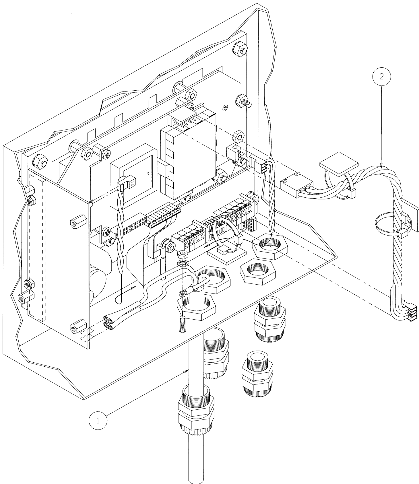
MSI-3550 METER FINAL ASSEMBLY 3550 BATTERY POWER Measurement Systems International 14240 Interurban Avenue South STE200 Seattle, Washington 98168-4661 U.S.A.
