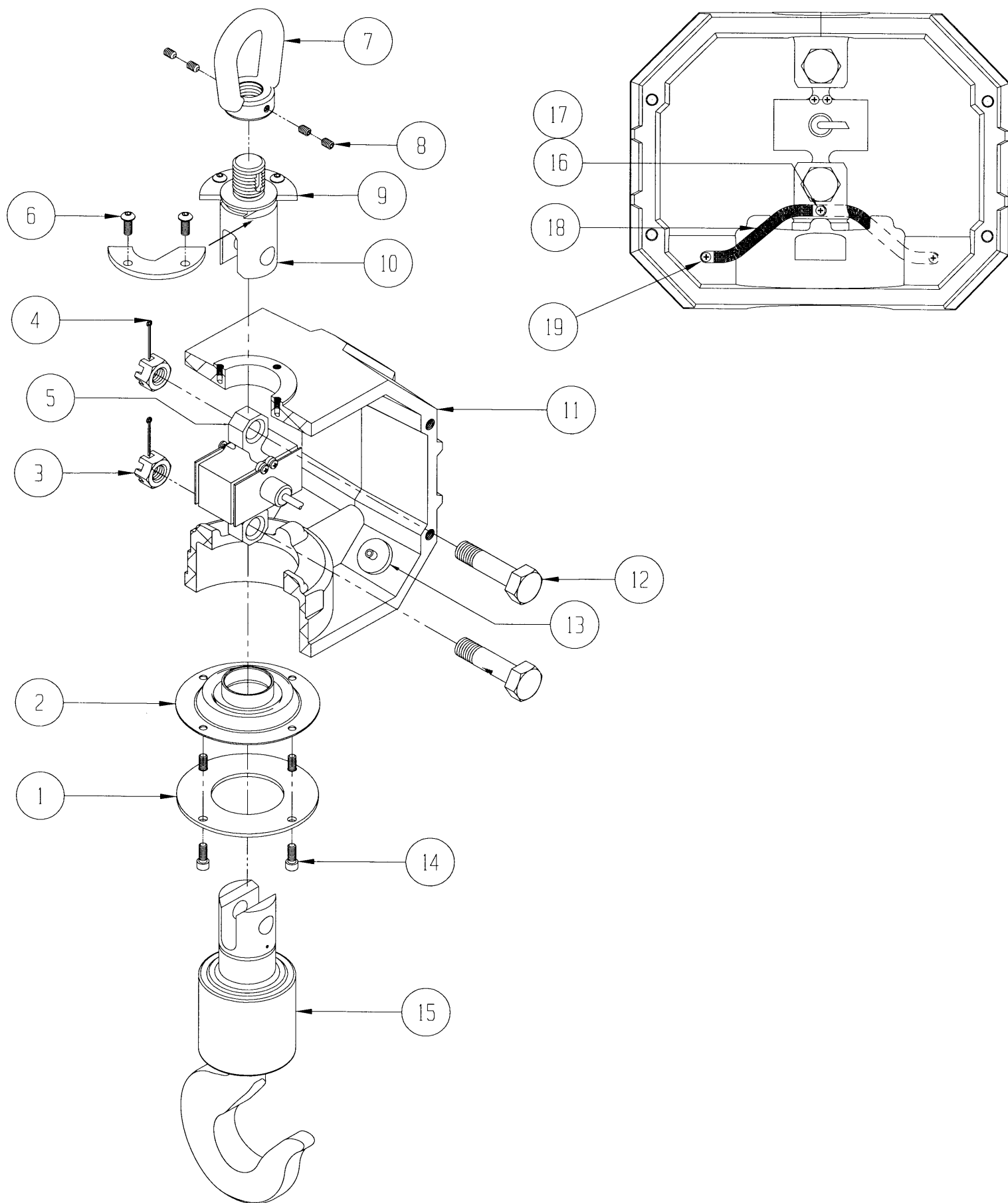
MSI-9300 PORTA-WEIGH PLUS RF MID-SECTION ASSEMBLY 500 THRU 10,000 LB Measurement Systems International 14240 Interurban Avenue South STE200 Seattle, Washington 98168-4661 U.S.A.
