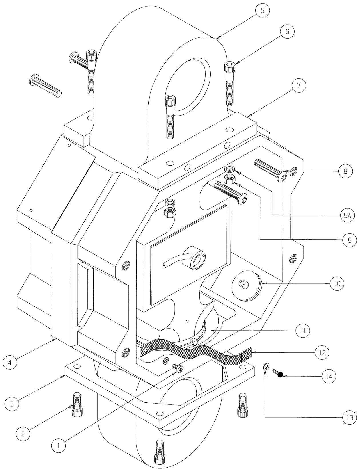
MSI-6260CS TRANS-WEIGH MID-SECTION ASSEMBLY - 50 & 70,000 LB Measurement Systems International 14240 Interurban Avenue South STE200 Seattle, Washington 98168-4661 U.S.A
