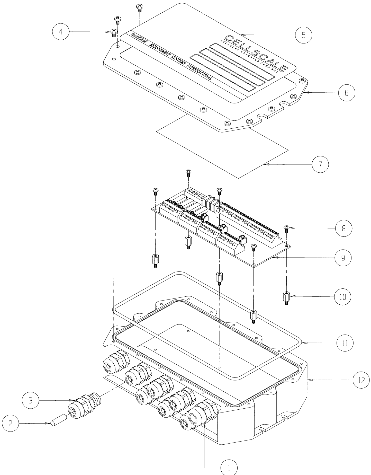
MSI-9002 CELLSCALE BREAKOUT/SUMMING BOX Measurement Systems International 14240 Interurban Avenue South STE200 Seattle, Washington 98168-4661 U.S.A.
