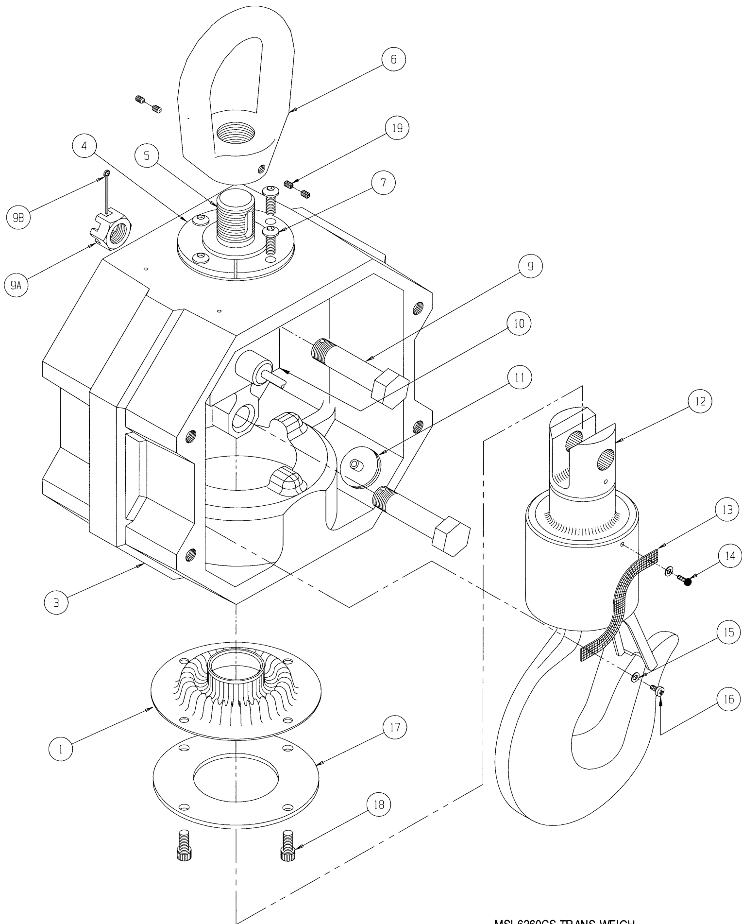
MSI-6260CS TRANS-WEIGH MID-SECTION ASSEMBLY 500 THRU 10,000 LB Measurement Systems International 14240 Interurban Avenue South STE200 Seattle, Washington 98168-4661 U.S.A.
