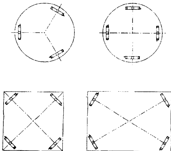
Typical mounting, 3 or 4 load cells Montage type 3 ou 4 cellules de pesage
