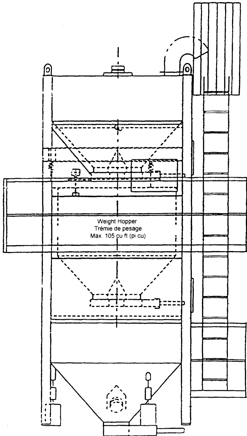
Figure 1: Typical Bulkweigher with weigh hopper
