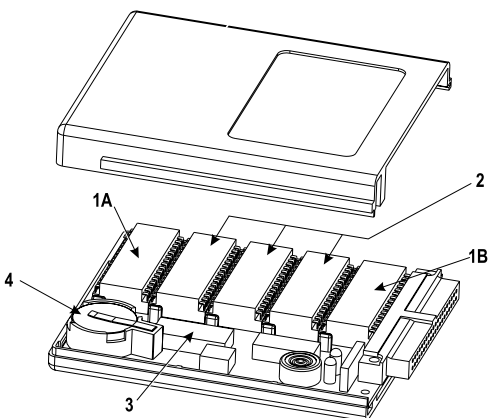
2D Bar Code Configuration
