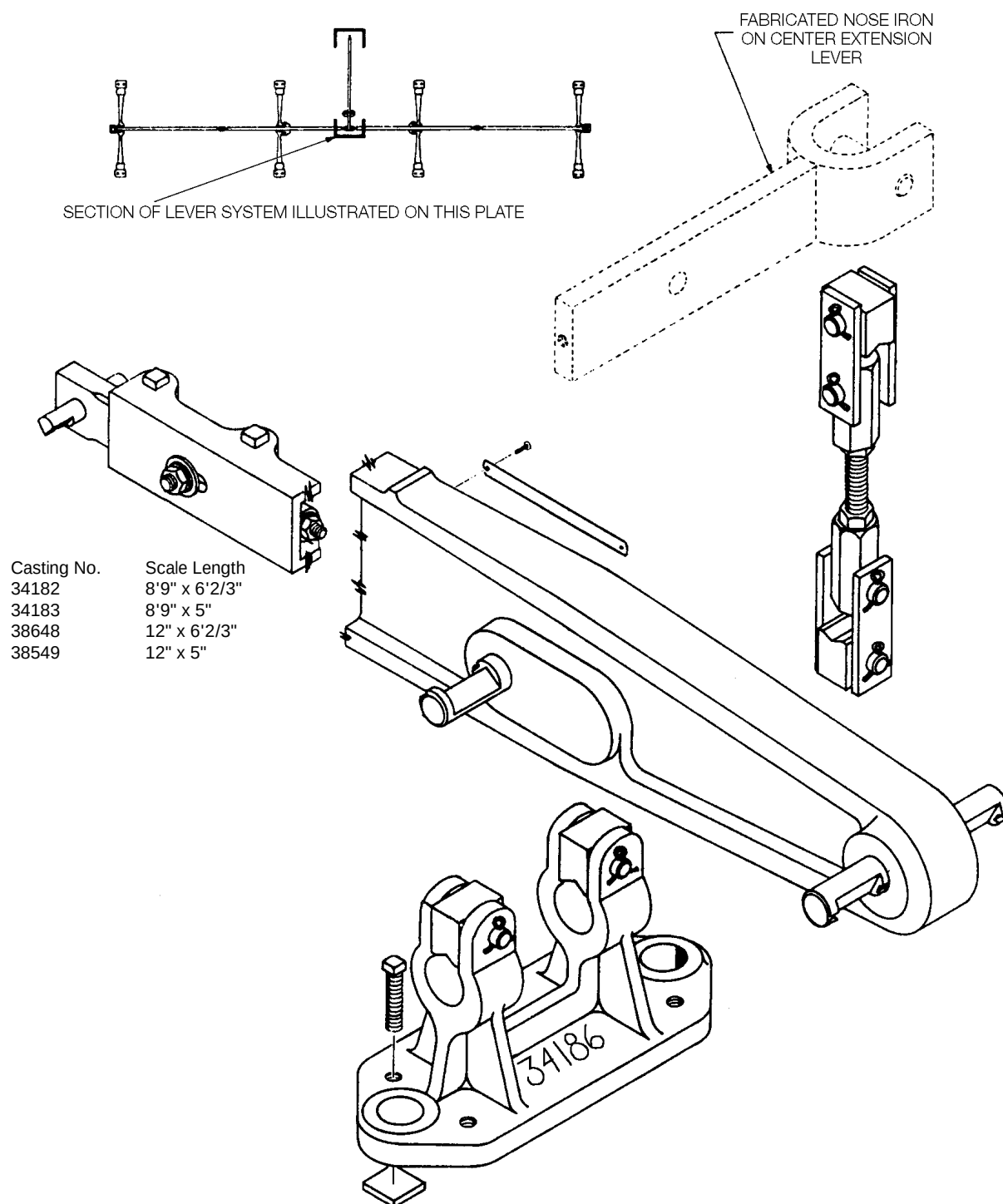
Transverse Lever (Cast), Stand & Connection Call with Casting No. for Price & Availability
